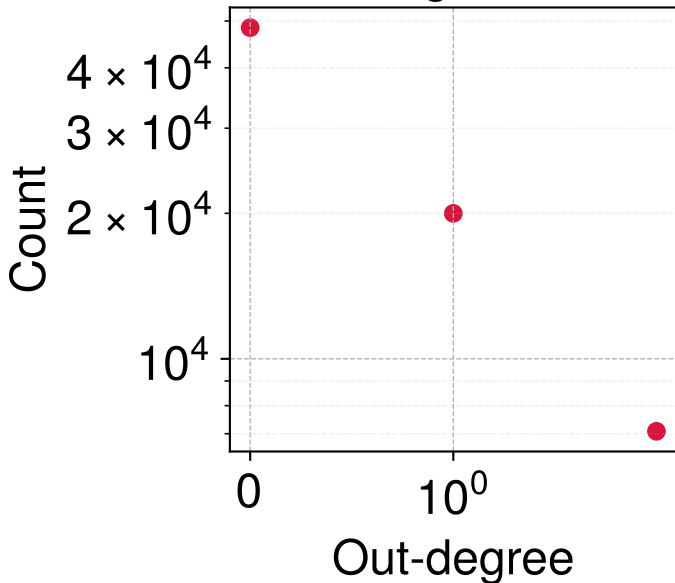
Payment Graph 3 out-degree dist.
