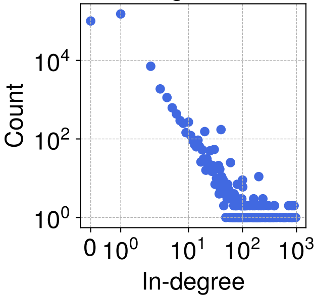
Payment Graph 4 in-degree dist.
