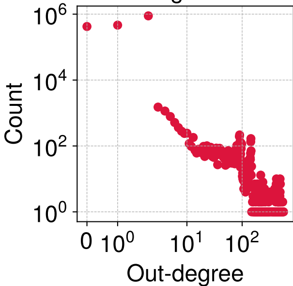
Payment Graph 5 out-degree dist.
