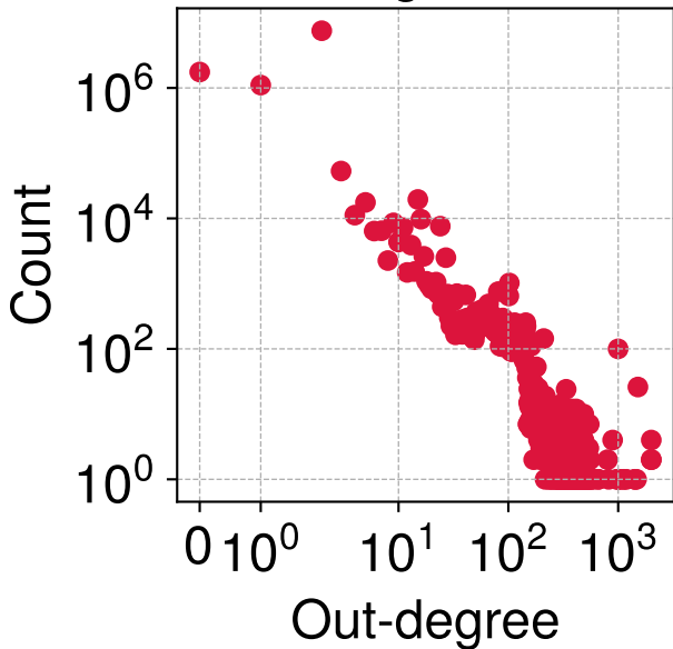
Payment Graph 7 out-degree dist.
