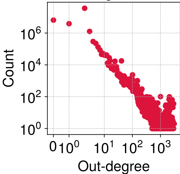
Payment Graph 9 out-degree dist.
