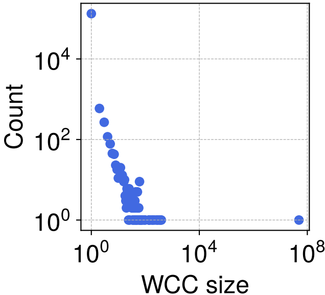
Payment Graph 9 WCC dist.
