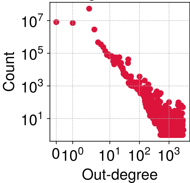
Payment Graph 10 out-degree distribution
