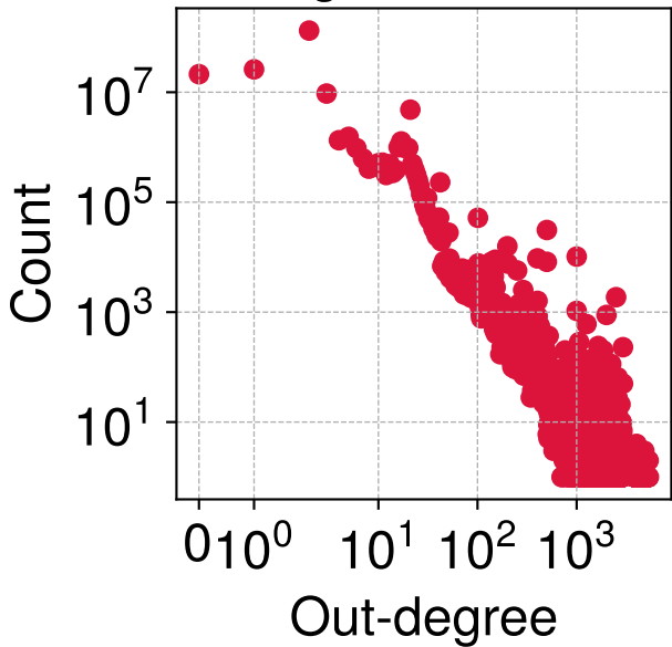
Payment Graph 13 out-degree distribution
