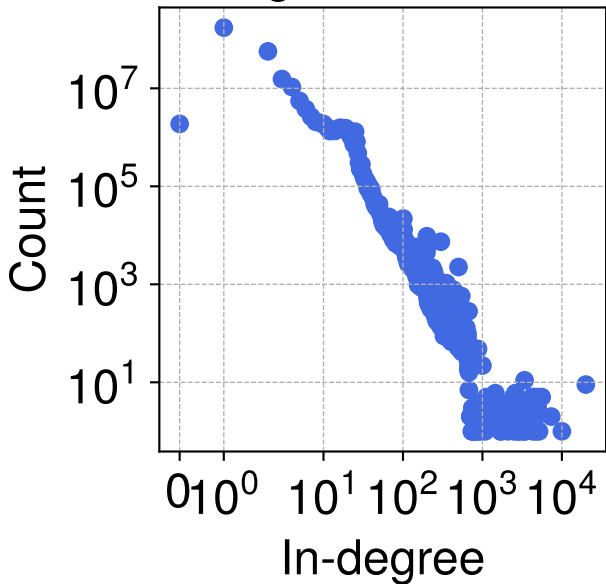
Payment Graph 14 in-degree distribution
