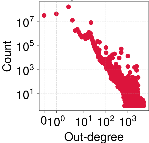
Payment Graph 14 out-degree distribution
