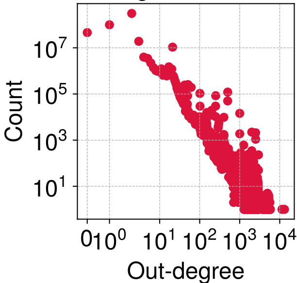
Payment Graph 16 out-degree distribution
