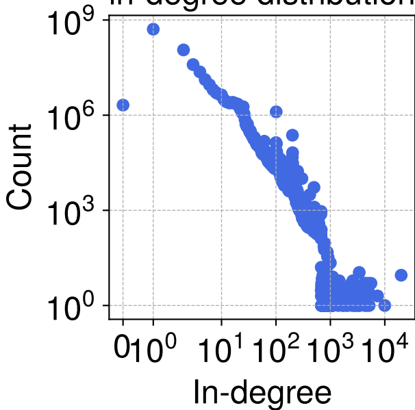
Payment Graph 18 in-degree distribution
