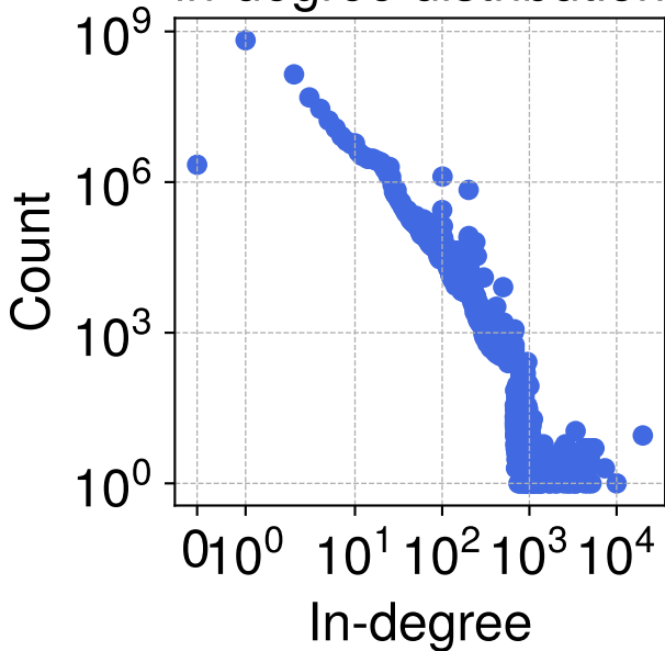
Payment Graph 20 in-degree distribution
