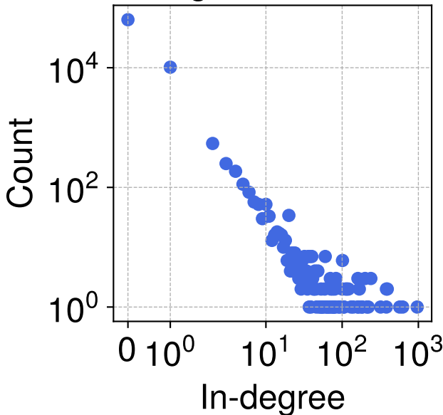
Payment Graph 3 in-degree distribution
