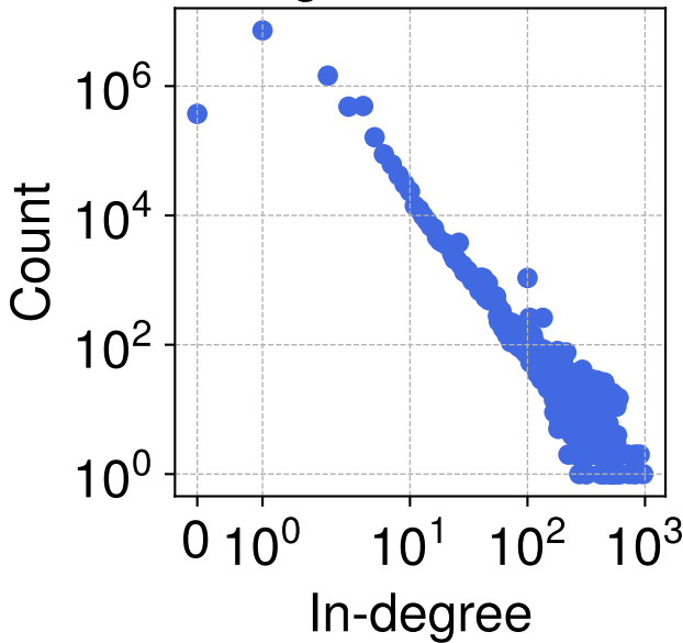
Payment Graph 7 in-degree distribution
