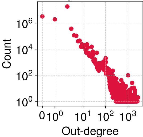
Payment Graph 8 out-degree distribution
