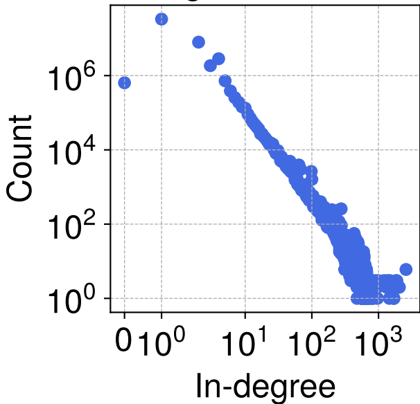
Payment Graph 9 in-degree distribution
