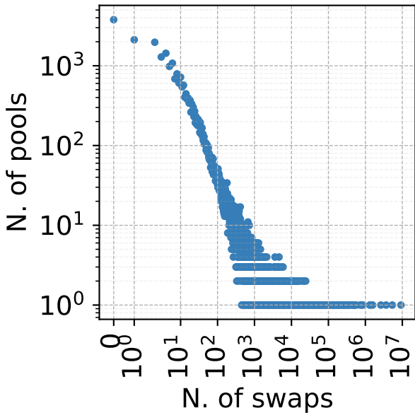
Swap distribution
