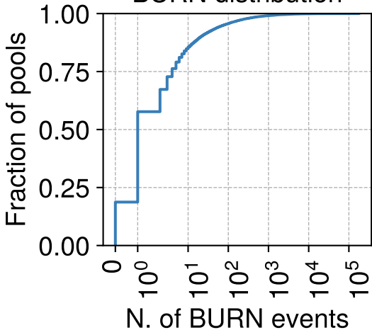
BURN distribution
