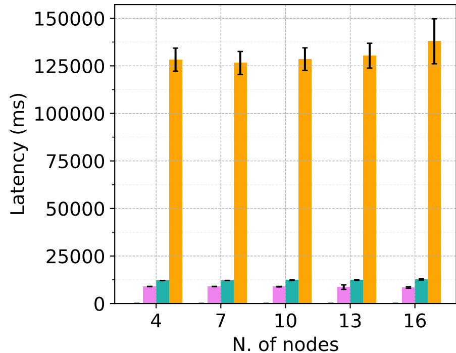
Latency breakdown: 30000 tokens, max. faulty nodes (alter)
