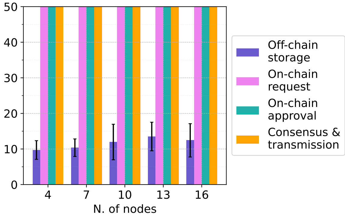
Latency breakdown: 3000 tokens, max. faulty nodes (timeout)
