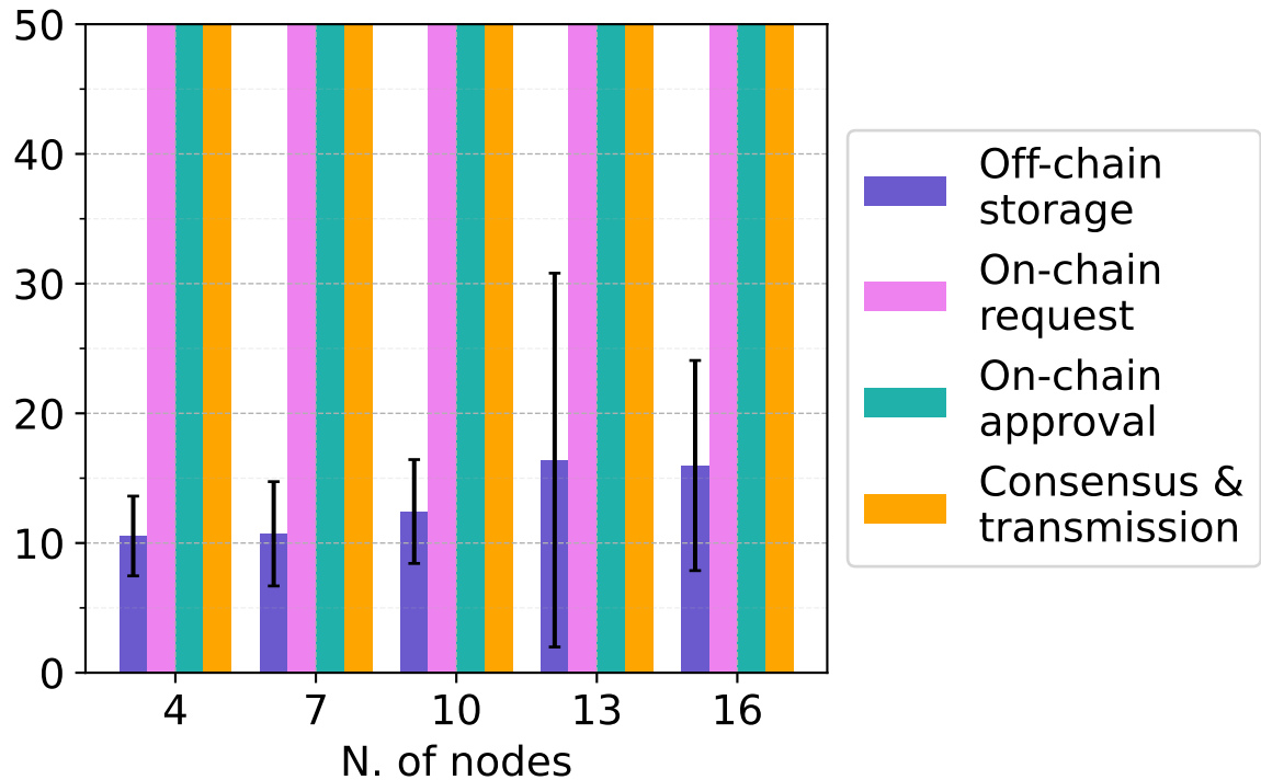
Latency breakdown: 30000 tokens, max. faulty nodes (timeout)
