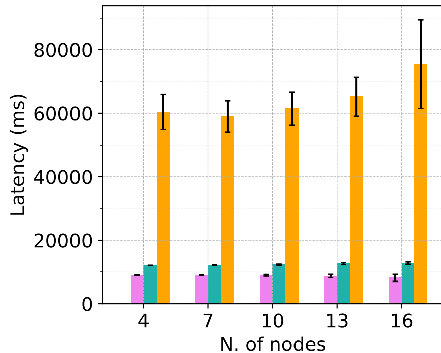
Latency breakdown: 3000 tokens, no faulty nodes
