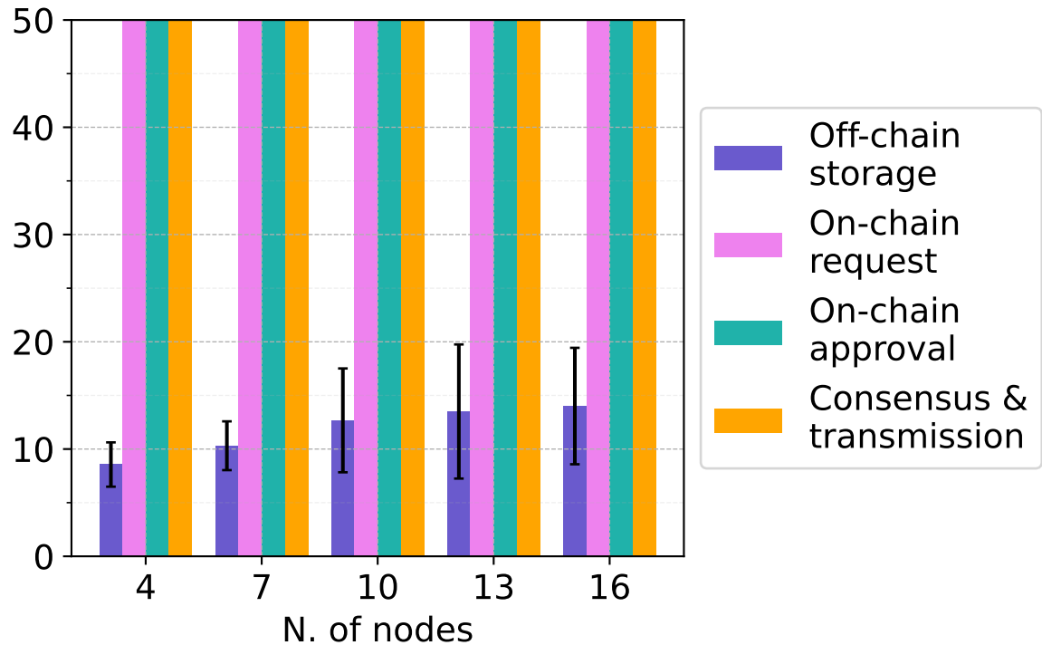
Latency breakdown: 30000 tokens, no faulty nodes
