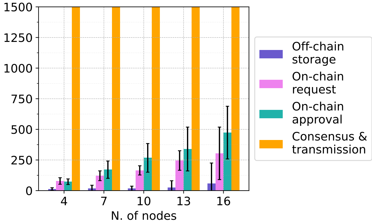
Latency breakdown: 30000 tokens, max. faulty nodes (timeout)
