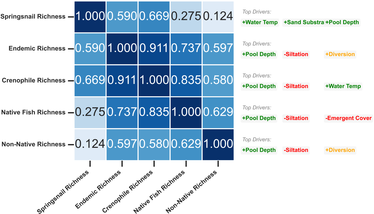
OLO Hierarchical Clustering of Biological Taxa Co-occurrence (Regional Aquifer stable thermal springs, N = 45)
