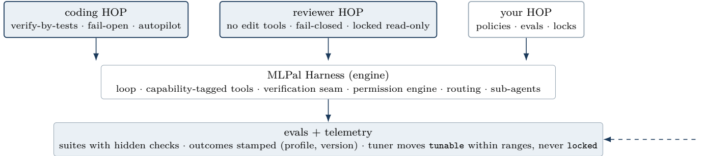
Figure 1. One engine, many HOPs. The artifact carries policy and its own definition of success; the engine enforces it; outcomes are attributable to a (profile, version) pair, closing the tuning loop as typed search.
