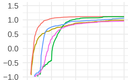
rbv2_rpart 14
