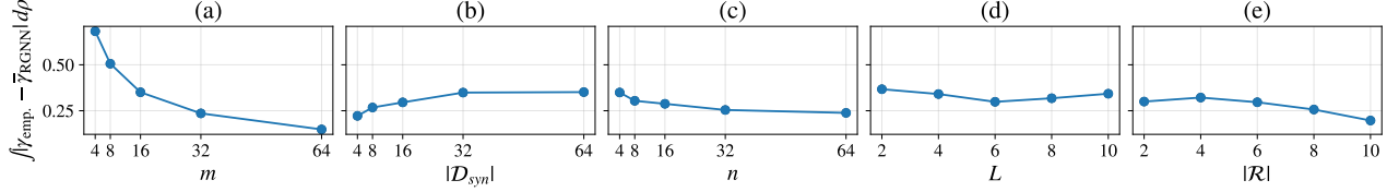
Figure 4. Tightness of \gamma_{RGNN} as model and dataset characteristics vary. Each panel reports the absolute area between \gamma_{empirical} and mean \bar{\gamma}_{RGNN} over a sparsity sweep, compare Figure 2 (a), so smaller area indicates a tighter bound. Panels vary (a) width m , (b) number of graphs |\mathcal{D}_{syn}| , (c) number of nodes per graph n , (d) number of message-passing layers L , and (e) number of relations |\mathcal{R}| . For each \rho , \gamma_{empirical} is estimated from 10 pruning-mask trials, while \gamma_{RGNN} is instantiated using model-specific statistics and averaged over 10 sparse-mask samples. Unless varied per panel: m = 16 , |\mathcal{D}_{syn}| = 30 , 6 nodes per graph, L = 3 , and |\mathcal{R}| = 3 .
