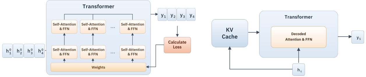
(a) Training: each token is used to calculate the loss for the position immediately after it
