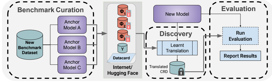
Figure 2. A contamination-resistant benchmark evaluation framework involves generating multiple projections at curation, and translation to the target model to be evaluated at discovery.
