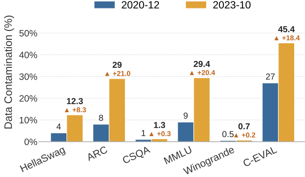
Figure 1. Detected contamination from 2020 to 2023 for various benchmark datasets (Figure is from (Li et al., 2024))
