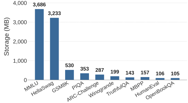
Figure 4. Approximate storage requirements for CRD projection of various existing benchmarks calculated based on number of test questions and average question token size using Llama2-7B and PyramidKV compression
