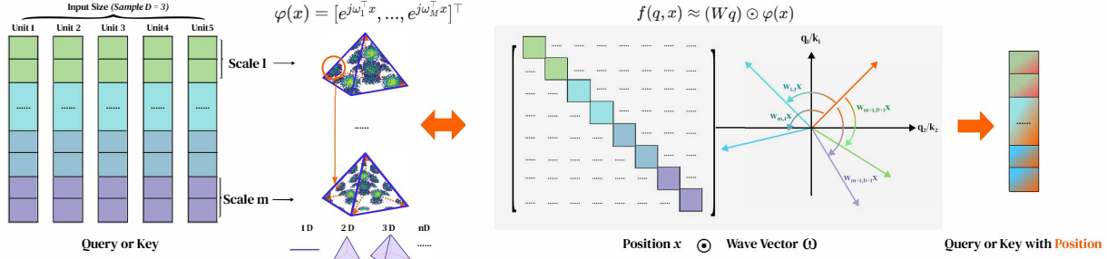
Figure 4. Visualization of the nD-RoPE implementation pipeline. Token coordinates x are projected onto multi-scale regular-simplex wave vectors \omega , producing phases \omega^T x . These phases generate rotary factors e^{j\omega^T x} , which are applied to query and key features while leaving the attention mechanism unchanged.
