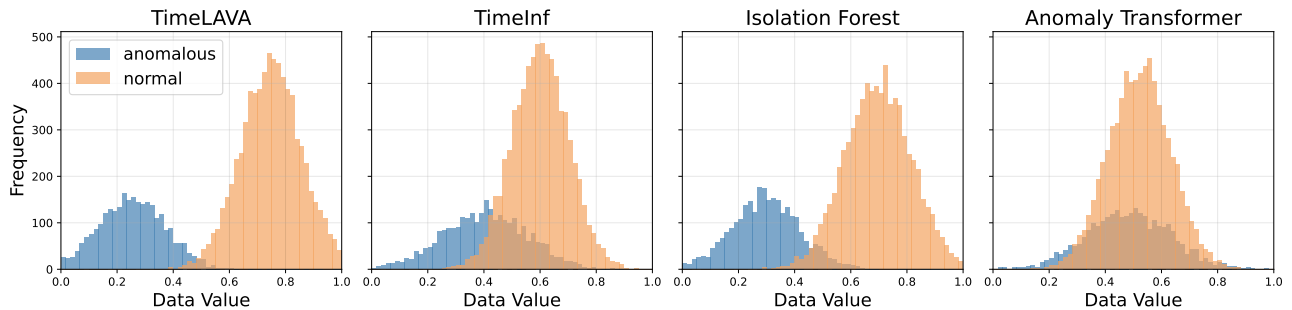
Figure 9. Anomaly score distributions. TimeLAVA achieves distinct separation between normal and anomalous segments, whereas baselines exhibit significant overlap.
