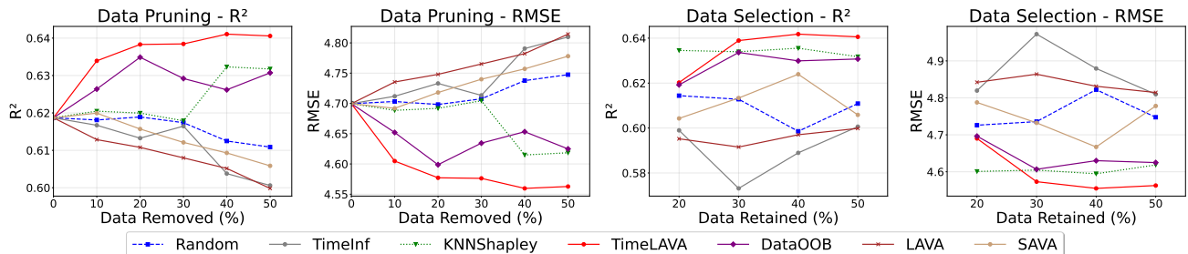
Figure 17. Data Selection and Pruning Results - ETTh1
