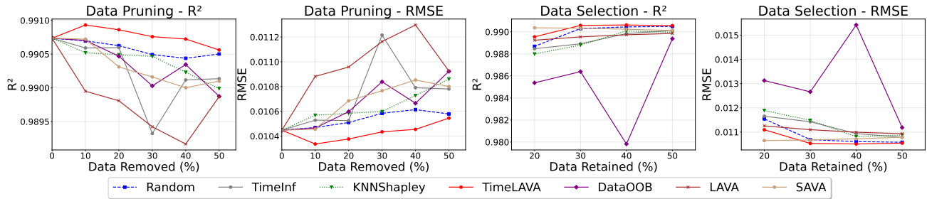
Figure 16. Data Selection and Pruning Results - Exchange
