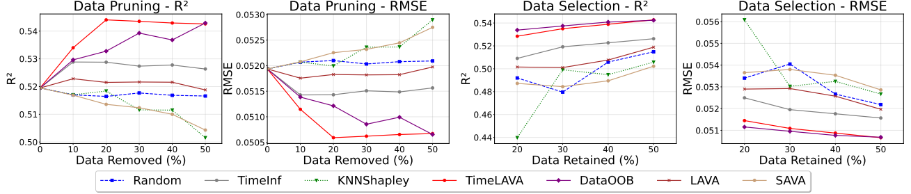
Figure 19. Data Selection and Pruning Results - Electricity
