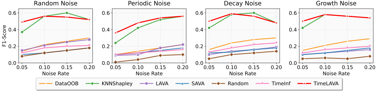
Figure 24. F1-score on Senior across different noise types.
