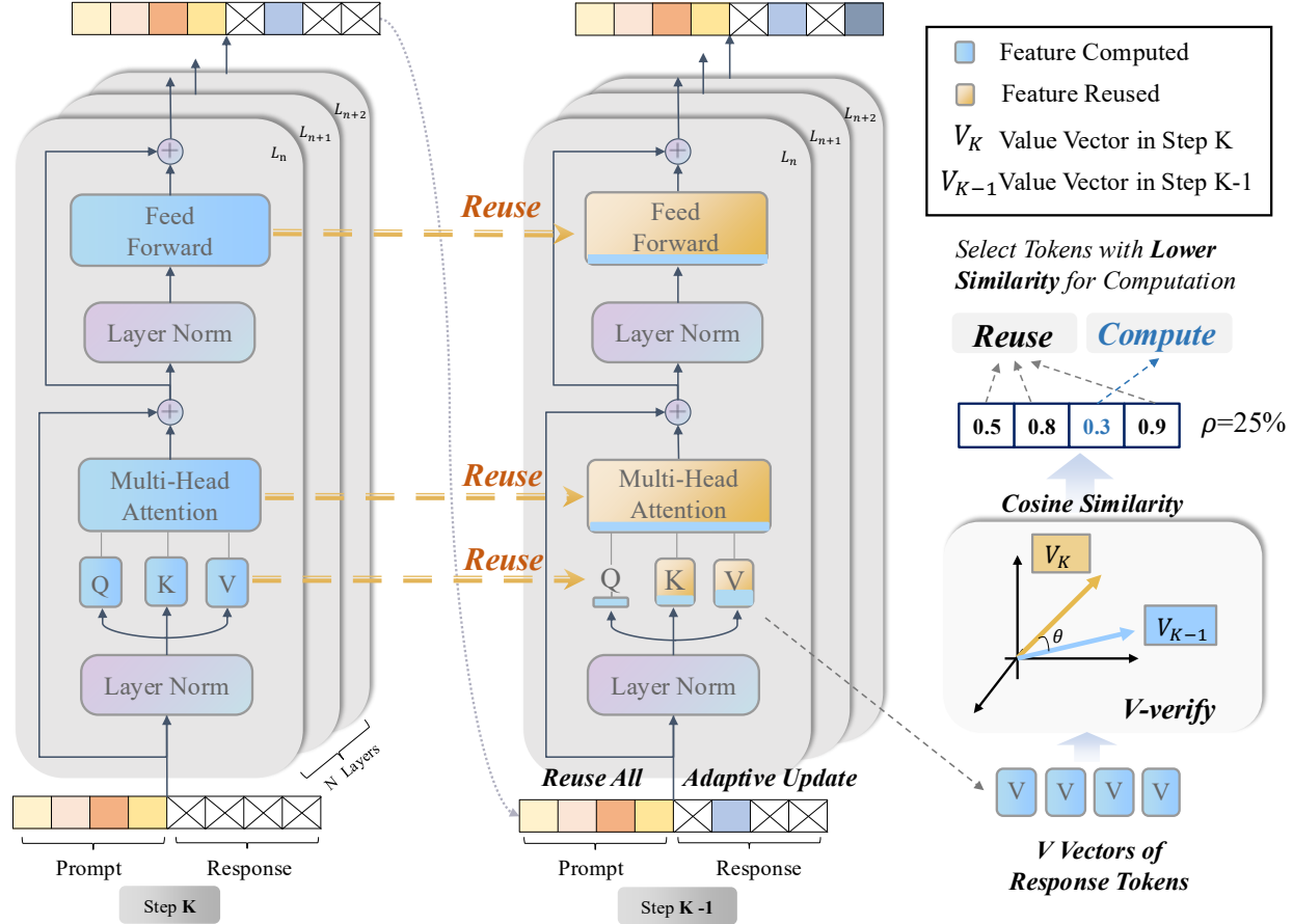
Figure 3. The dLLM-Cache pipeline. Prompt features are updated at long intervals, while response features are fully recomputed every K_r steps and otherwise only the tokens least similar to cached V are recomputed.
