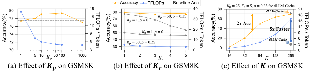
Figure 5. (a) Varying K_p with K_r = 1, \rho = 0 . (b) Varying K_r under two settings: baseline ( K_p = 1, \rho = 0 , gray) and our setup ( K_p = 50, \rho = 0.25 in Table 1). (c) Varying the denoising steps K for the uncached baseline. The gray marker denotes dLLM-Cache with K_p = 25, K_r = 5, \rho = 0.25 . dLLM-Cache achieves a better Pareto optimum: about 5\times faster than the standard 256-step baseline at similar accuracy, and over 2\times more accurate than a baseline with equal FLOPs. (a–b) LLaDA Instruct; (c) LLaDA Base.
