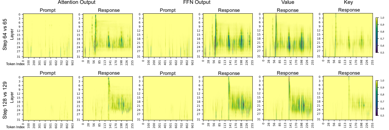
Figure 1. Cosine similarity of Key, Value, Attention Output and FFN Output between two adjacent denoising steps in a dLLM, highlighting computational redundancies. The heatmaps show similarity across adjacent steps for prompt and response tokens, respectively, where a lighter color indicates a higher similarity of a token compared with its value in the last step. These results demonstrate: (I) The prompt region exhibits high similarity, while the response region shows different similarity in different tokens. (II) Notably, only a small fraction of response tokens exhibit significantly lower similarity, suggesting that selective recomputation is sufficient. (III) Response tokens’ value similarity closely aligns with attention and FFN output similarity, supporting that value changes can serve as an effective indicator to identify those most changed response tokens.
