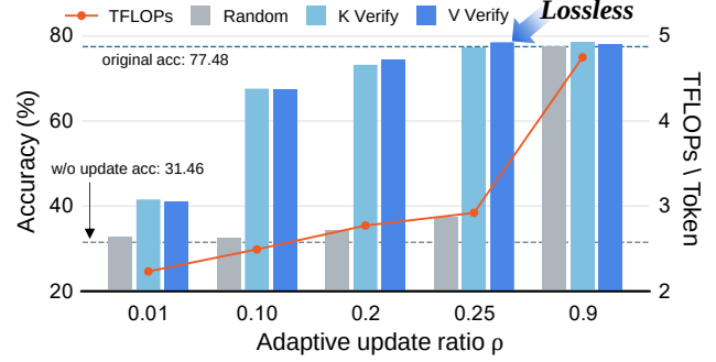
Figure 4. Effect of token selection strategy on GSM8K using LLaDA 8B Instruct model under varying update ratios \rho .
