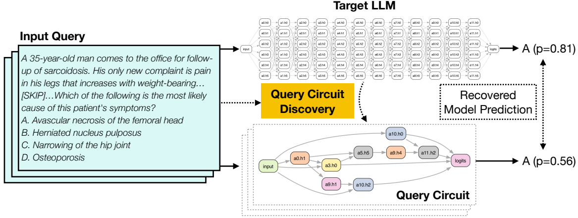
Figure 1. Query circuit discovery aims to identify a sparse sub-network within the LLM that underlies the model response to a user input query. The LLM and circuit in this illustration are simplified for visualization.
