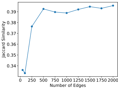
(a) Averaged Jaccard similarity between the capability circuit and query circuits.
