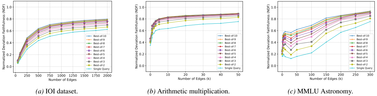
Figure 7. Performance of BoN sampling with different numbers of paraphrases. As BoN selects the most faithful circuit, its performance exhibits monotonically increasing yet diminishing returns.
