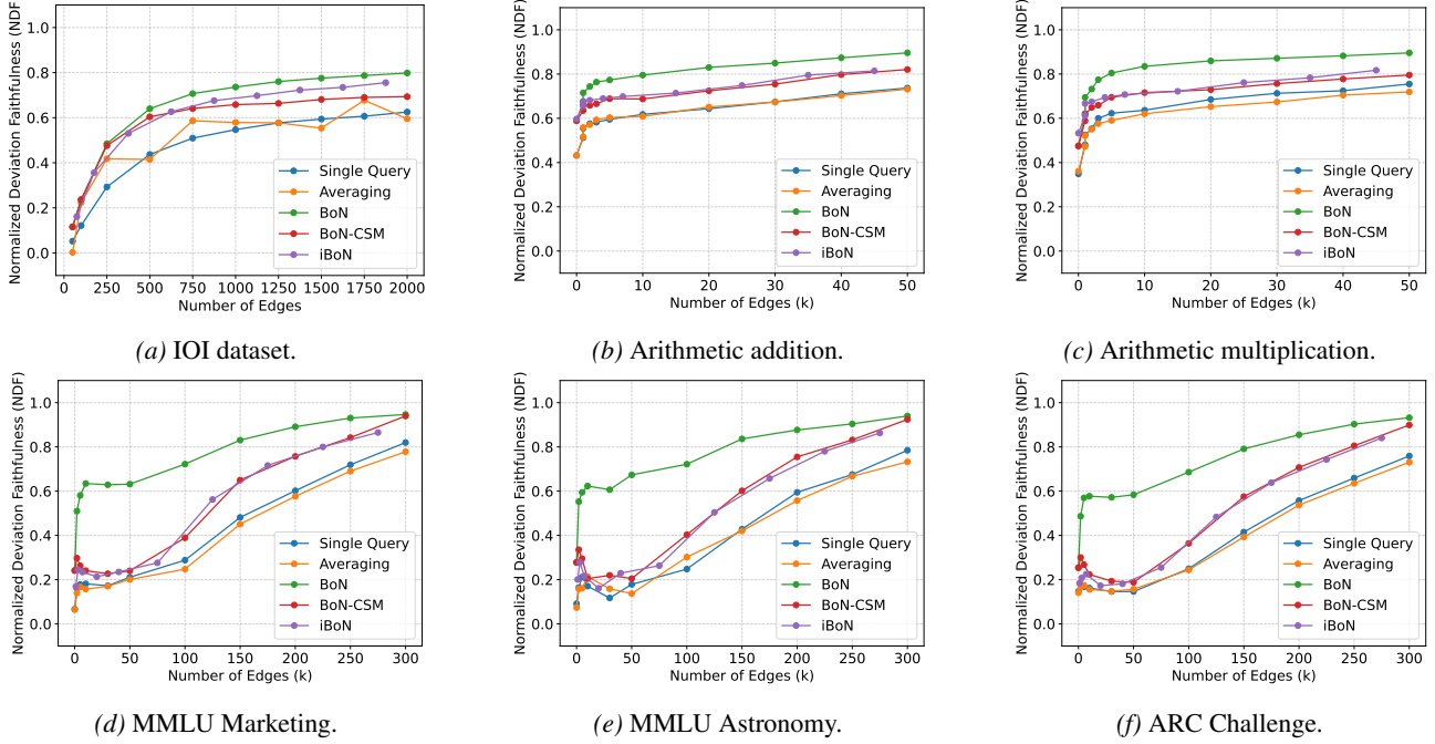
Figure 6. Main results of BoN sampling for query circuit discovery. BoN substantially outperforms all other methods. Although iBoN and BoN-CSM, two fast approximations to BoN, perform worse than it, they still clearly exceed both baselines.
