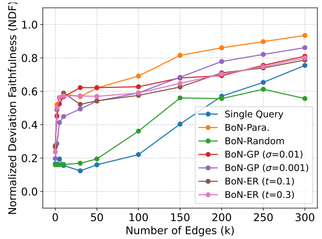
(b) MMLU Astronomy.
