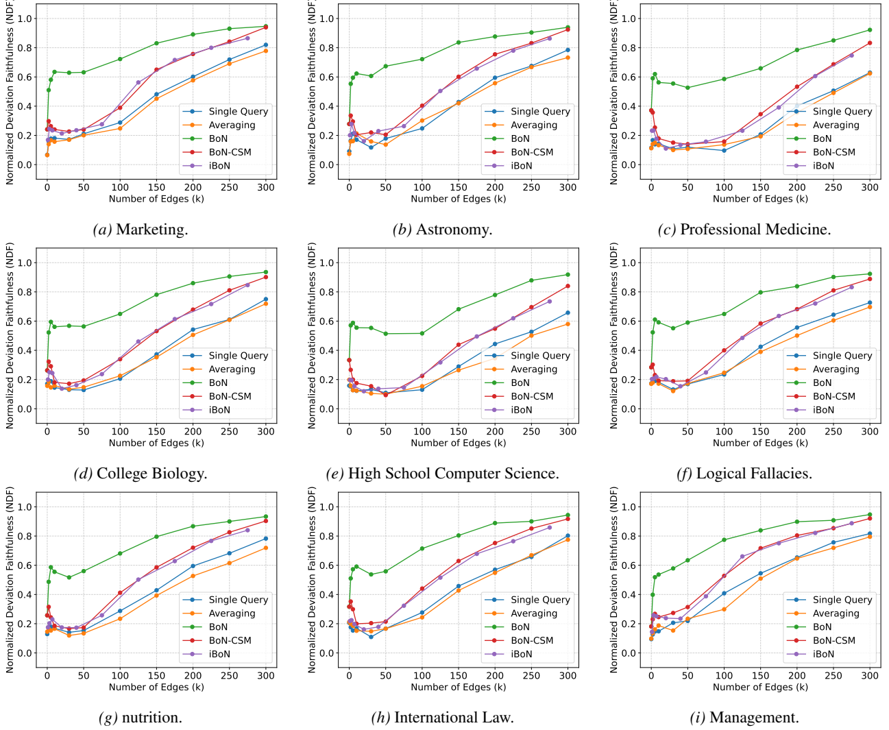
Figure A12. Complete results of BoN sampling for query circuit discovery on nine MMLU categories.
