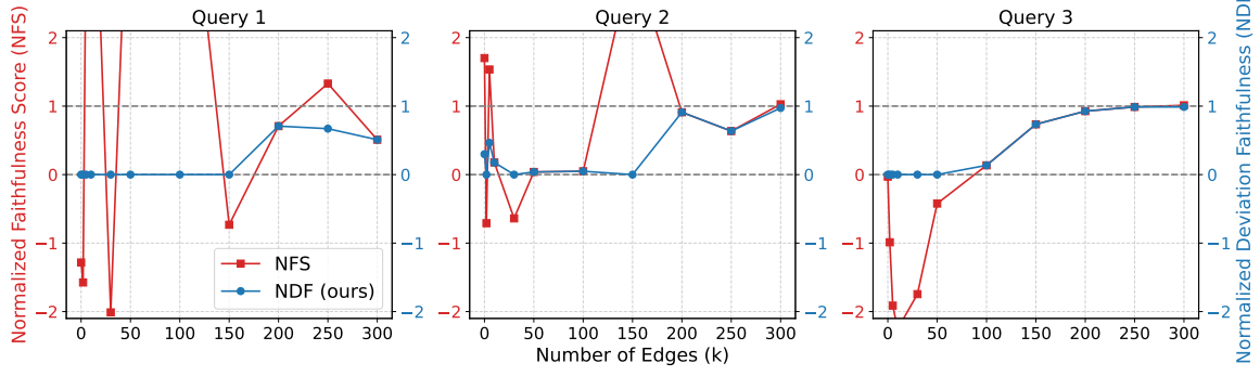
Figure 3. Complete evaluation results for the three queries adopted in Figure 2a and Table 1.
