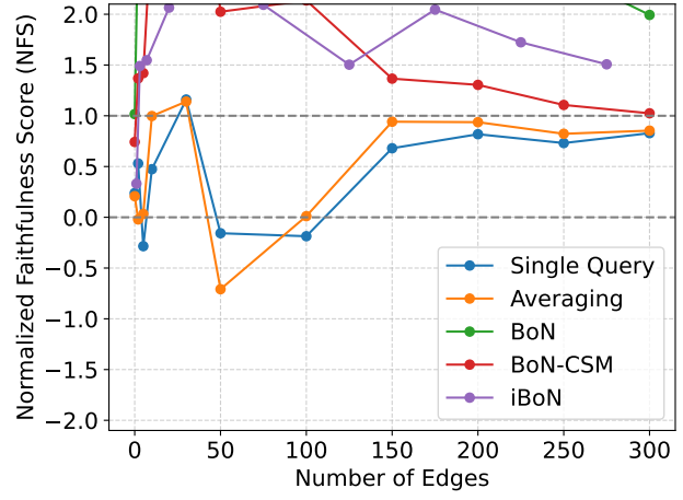
(b) MMLU Astronomy.
