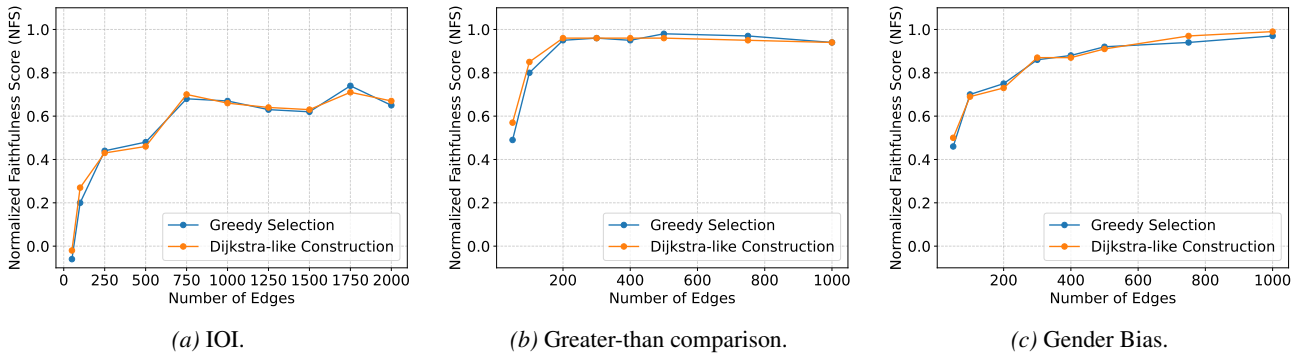
Figure A15. Performance comparisons between greedy selection and Dijkstra-like iterative construction for forming a circuit. The two methods achieve similar results on all three tested datasets.
