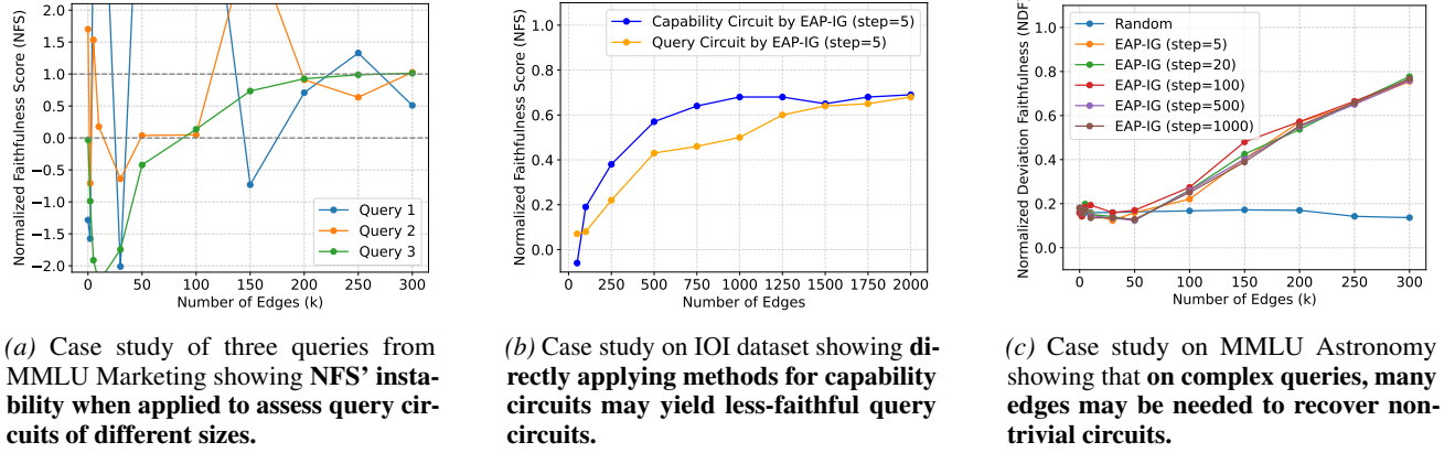
Figure 2. Technical challenges of query circuit discovery.
