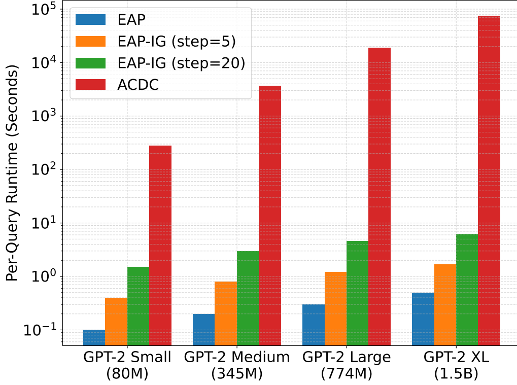
Figure A16. Per-query edge scoring runtime of activation patching (ACDC) versus attribution patching (EAP and EAP-IG) methods. The dataset is IOI. Runtime of ACDC easily grows to hours.
