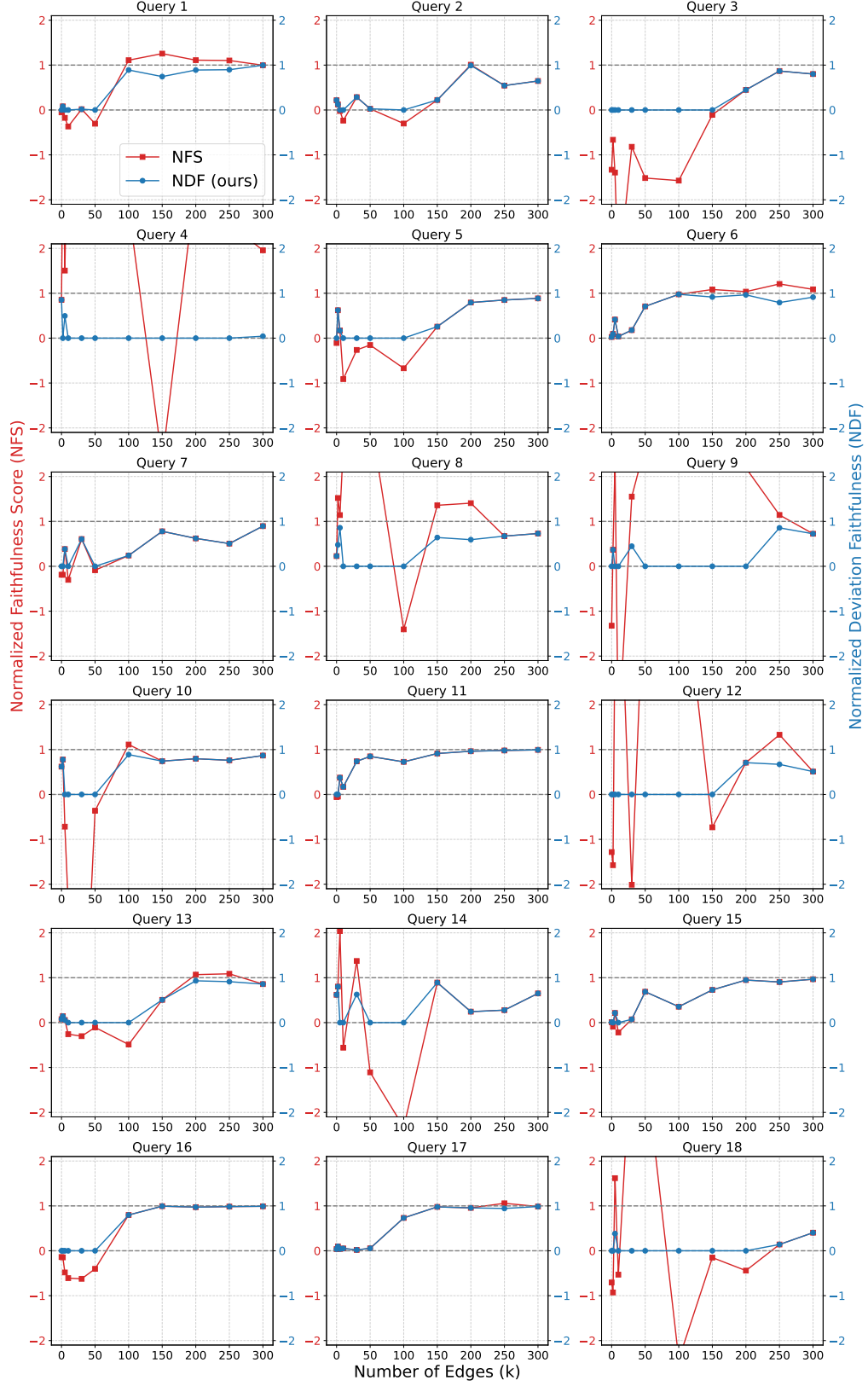
Figure A9. More query circuit evaluation results using NFS and our proposed NDF, which provides more stable evaluation and can better track the discovery progress as the circuit size grows.
