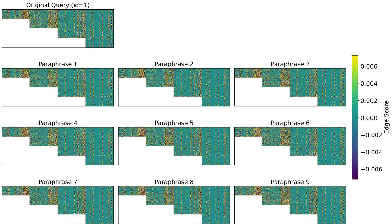
Figure A11. Edge score matrices of a query and its nine paraphrases in MMLU Astronomy. EAP-IG is used to calculate the score of each edge (i.e., each entry in the matrix). These matrices share similar patterns, and are dissimilar to those in Figure A10.
