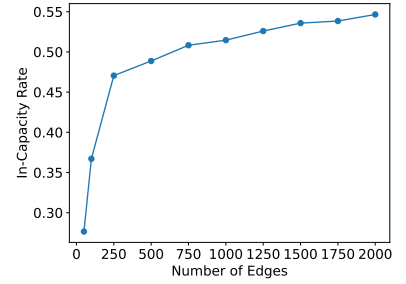
(c) Averaged percentage of edges in query circuits that also appear in the capability circuit.
