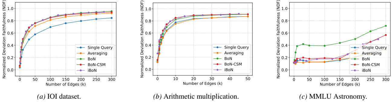
Figure A14. Scaling BoN sampling for query circuit discovery to larger models (GPT-2 XL for IOI; Llama-3-8B-Instruct for arithmetic multiplication and MMLU astronomy). BoN, iBoN, and BoN-CSM still consistently outperform both baselines.
