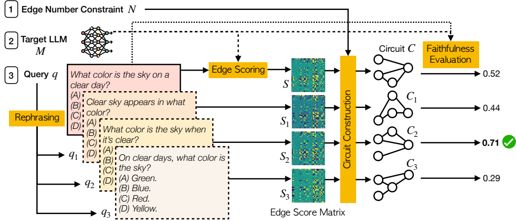
Figure 5. The pipeline of Best-of-N sampling for discovering a faithful query circuit of N edges for an input query q , for which it generates p paraphrases. p = 3 in this illustration.
