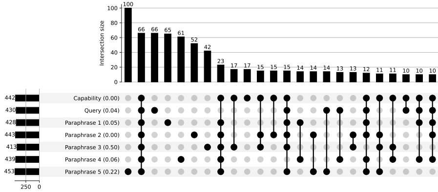
Figure 8. UpSet plot of the capability circuit and query circuits of a randomly selected query discovered by it or its paraphrases. A total of 66 edges are shared across all circuits.
