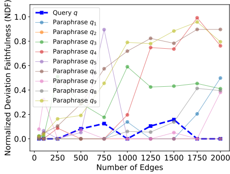
Figure 4. A case study on IOI dataset. Circuits discovered by the original input query’s paraphrases may recover model performance on the query.
