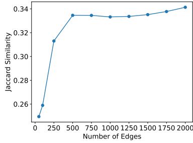
(b) Averaged Jaccard similarity among the circuits derived from a query and its paraphrases.
