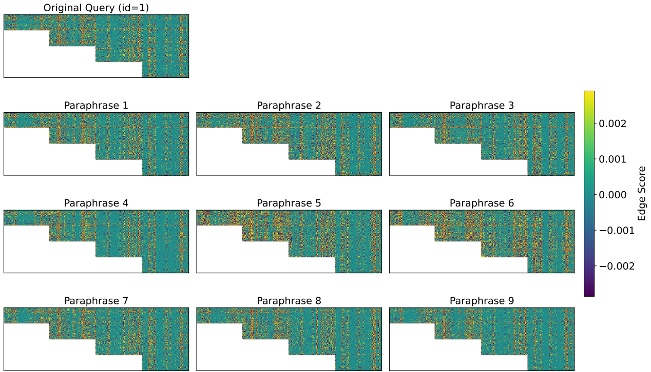
Figure A10. Edge score matrices of a query and its nine randomly selected paraphrases in IOI. EAP-IG is used to calculate the score of each edge (i.e., each entry in the matrix). These matrices share similar patterns.
