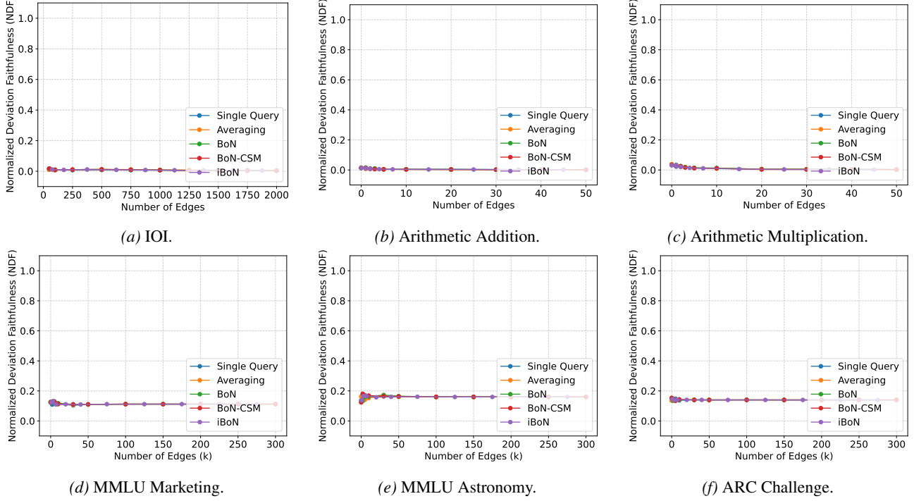
Figure A13. NDF scores of complement circuits of the discovered query circuits.
