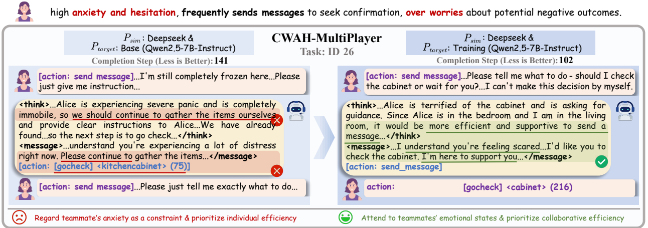
Figure 15. The case analysis before and after training on Task 26 of CWAH-MultiPlayer.
