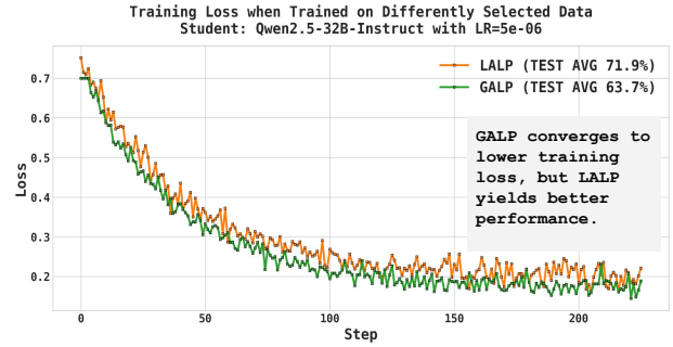
Figure 6. Training loss when fine-tuning on differently selected data (student: Qwen2.5-32B-Instruct). Global selection achieves lower training loss, but local selection yields higher downstream reasoning accuracy, illustrating a loss-generalization mismatch.
