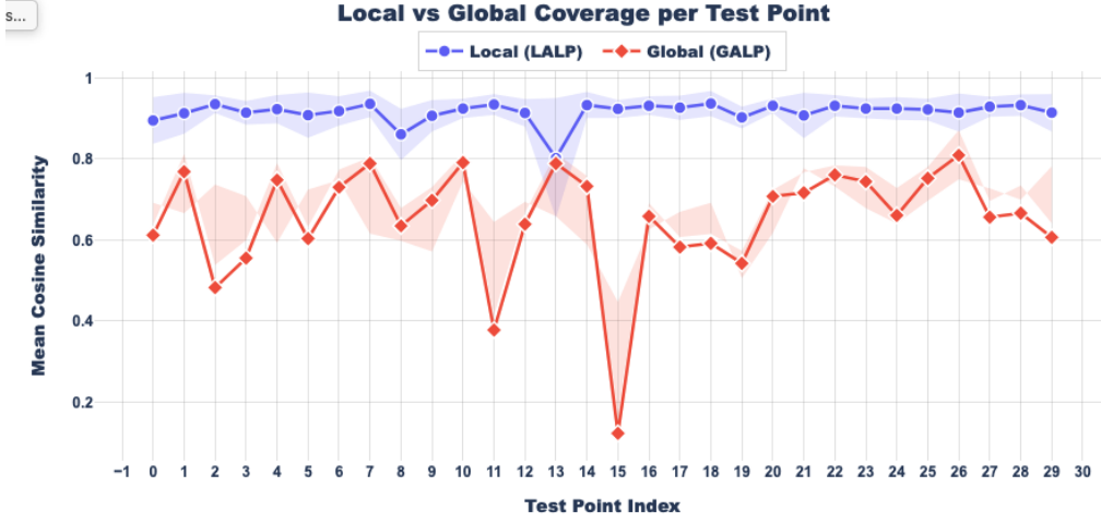
Figure 7. AMC Test Points
