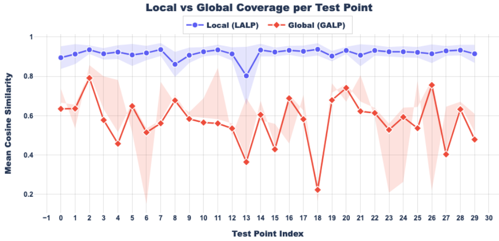
Figure 8. GSM8K Test Points
