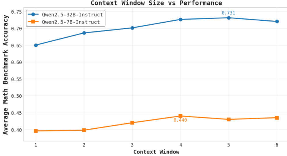
Figure 9. Context window size vs performance. Ablation on two student models.
