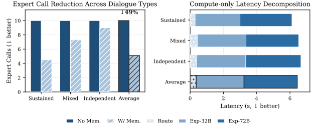
Figure 2. Efficiency analysis. Left: expert-call reduction across dialogue types when enabling cross-modal memory (avg. 49%). Right: compute-only latency decomposition; expert inference dominates while routing and orchestration overhead remain small. Here, T_{\text{route}} includes controller inference, token parsing/validation, memory lookup (when enabled), and scheduling, and the same measurement scope is used across settings for a fair overhead comparison. Overhead is computed as 100 \times \frac{T_{\text{route}}}{T_{\text{route}} + T_{\text{Exp-72B}}} and stays below 12% across scenarios (avg. 10.36%).
