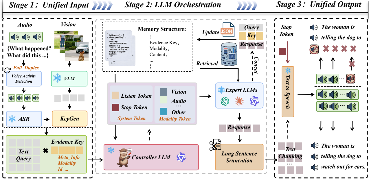
Figure 1. Overview of our training-free MLLM Orchestration pipeline. Stage 1 normalizes multimodal inputs into a unified representation with evidence keys. Stage 2 uses a controller to emit closed-vocabulary control tokens, routes to external experts, and performs cache-or-call retrieval with evidence-keyed memory. Stage 3 streams ordered outputs and supports barge-in by canceling pending jobs.
