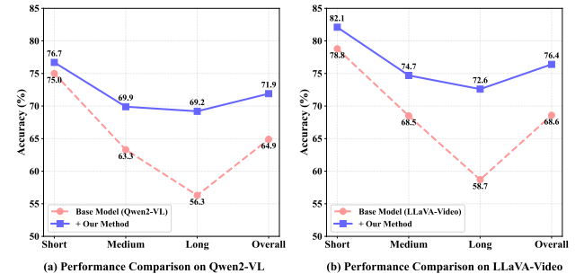
Figure 3. Video-MME accuracy stratified by video length. Our orchestration consistently improves over the corresponding single-model baseline under the same backbone, with larger gains on longer videos, indicating that protocol-driven routing and evidence aggregation are particularly beneficial when temporal context grows. (a) Qwen2-VL backbone. (b) LLaVA-Video backbone.
