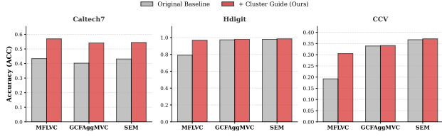
Figure 7. Comparison of the ACC of the policy model as a plug-and-play module across three baselines.
