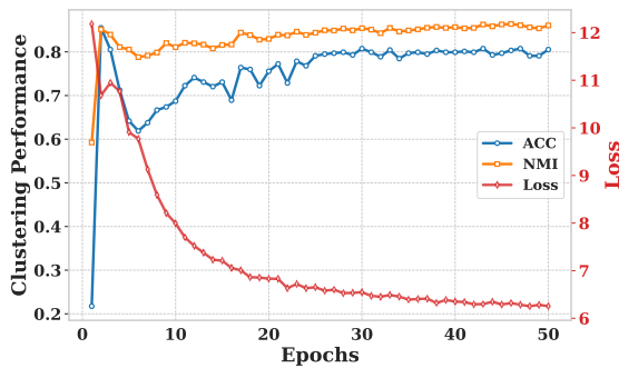
Figure 9. Convergence analysis.
