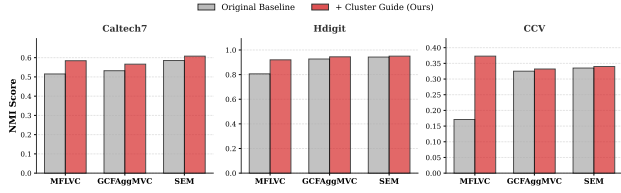
Figure 8. Comparison of the NMI of the policy model as a plug-and-play module across three baselines.
