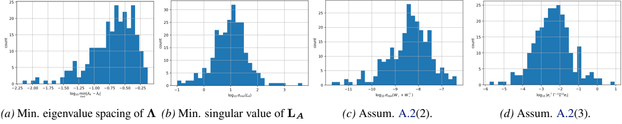
Figure 4. Numerical probe of spectral/rank assumptions: a) The histogram of minimum pairwise eigenvalue spacing of \Lambda . b) The histogram of minimum singular of L_A . c) The condition in Assumption A.2(2) d) The condition in Assumption A.2(3) (The values on the x-axis are in \log_{10} scale)
