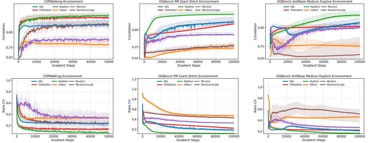
Figure 3. (Top) Pearson correlation coefficients and (Bottom) coefficient of variation ratios across a selection of test environments. Shaded regions show the range of values across five random seeds, with upper and lower boundaries representing maximum and minimum values.
