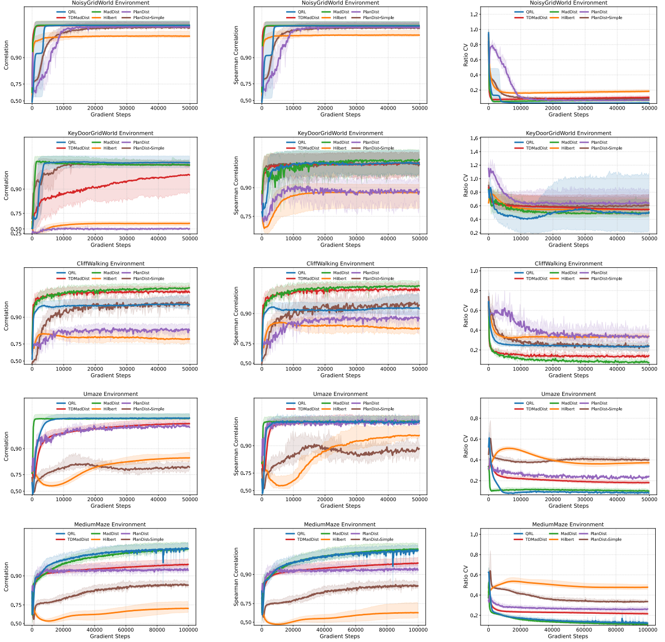
Figure 14. Pearson and Spearman correlation coefficients and coefficient of variation (CV) ratios across the NoisyGridWorld, KeyDoorGridWorld, CliffWalking, Umaze, and MediumMaze environments. Shaded regions show the range of values across five random seeds, with upper and lower boundaries representing maximum and minimum values.
