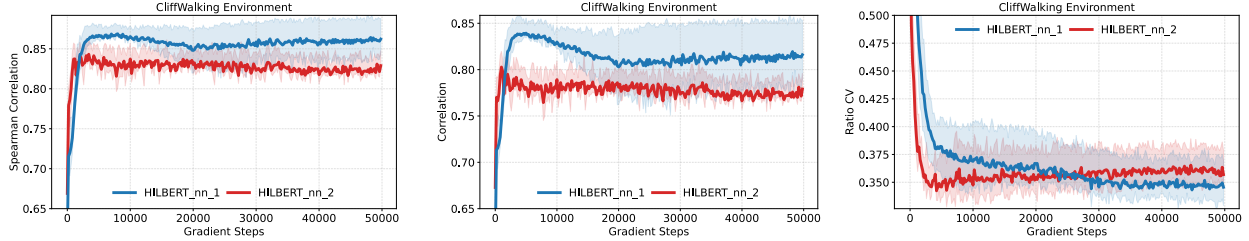
Figure 9. Impact of neural network size on Spearman correlation, Pearson correlation, and Ratio CV for the Hilbert algorithm in the CliffWalking environment. Shaded regions show the range of values across five random seeds, with upper and lower boundaries representing maximum and minimum values.
