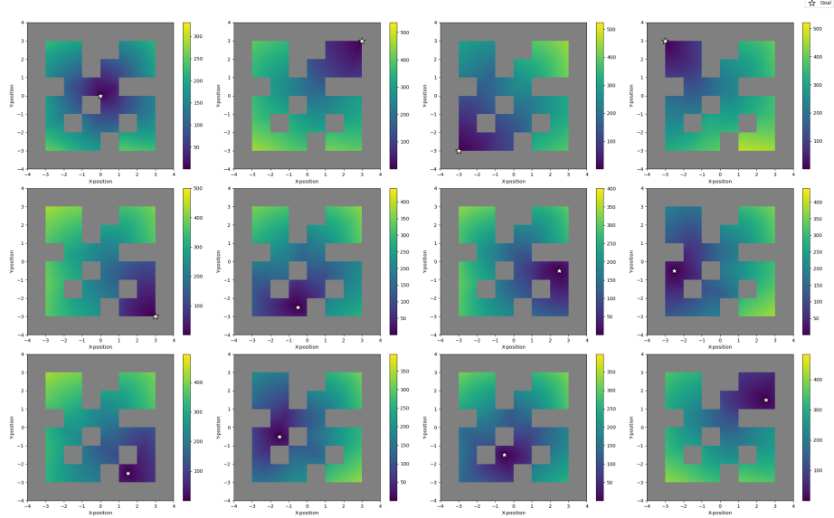
Figure 13. Visualization of the learned MAD landscape using MadDist on the MediumMaze environment. The heatmap represents the predicted distance from a fixed goal state to every other point in the maze
