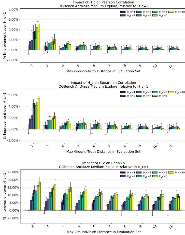
Figure 12. Impact of H_c on Pearson and Spearman correlation coefficients and coefficient of variation (CV) ratios on ogbench AntMaze Medium Explore
