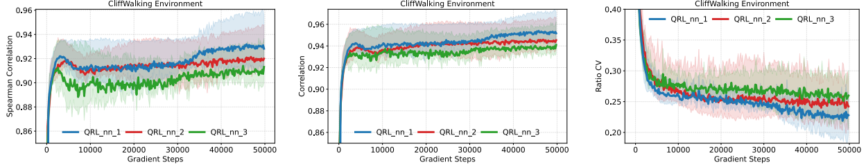
Figure 8. Impact of neural network size on Spearman correlation, Pearson correlation, and Ratio CV for the QRL algorithm in the CliffWalking environment. Shaded regions show the range of values across five random seeds, with upper and lower boundaries representing maximum and minimum values.
