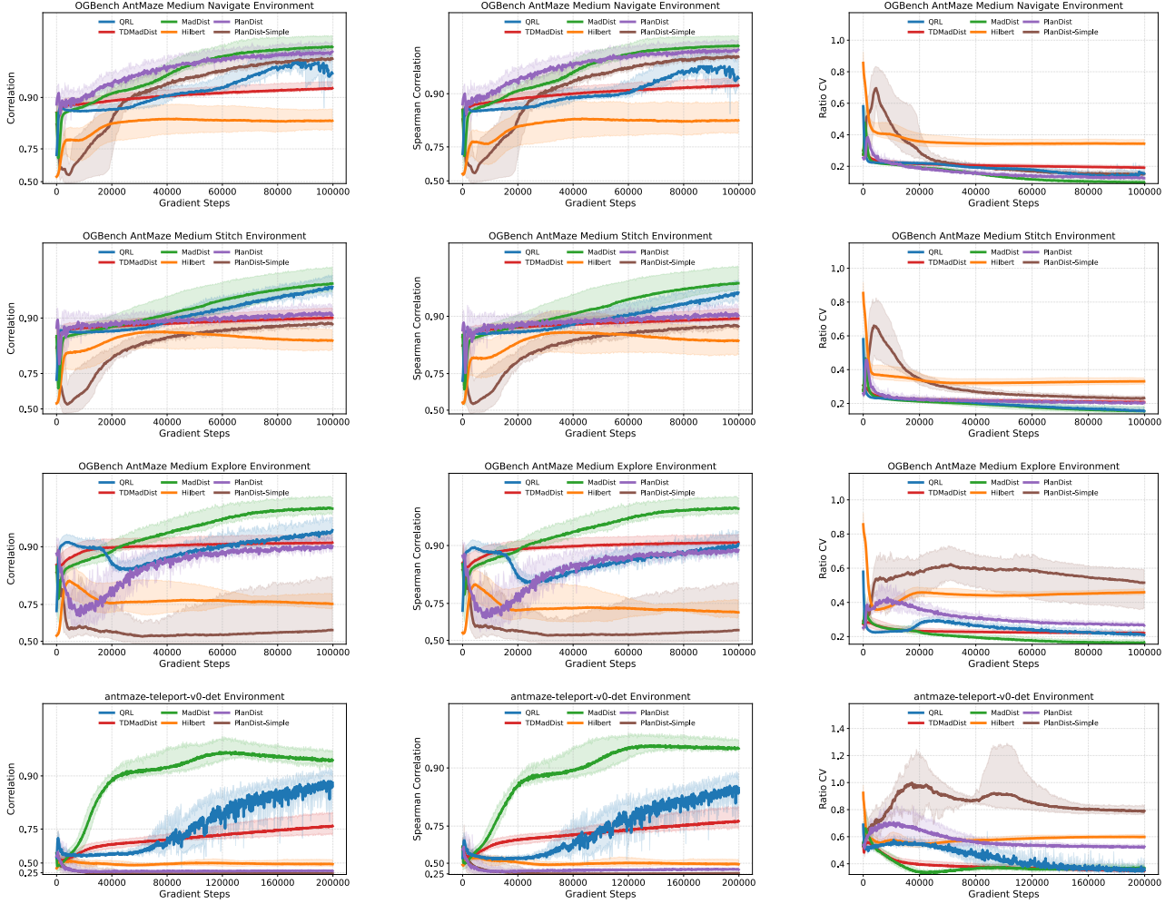
Figure 16. Pearson and Spearman correlation coefficients and coefficient of variation (CV) ratios across OGBench AntMaze test environments. Shaded regions show the range of values across five random seeds, with upper and lower boundaries representing maximum and minimum values.
