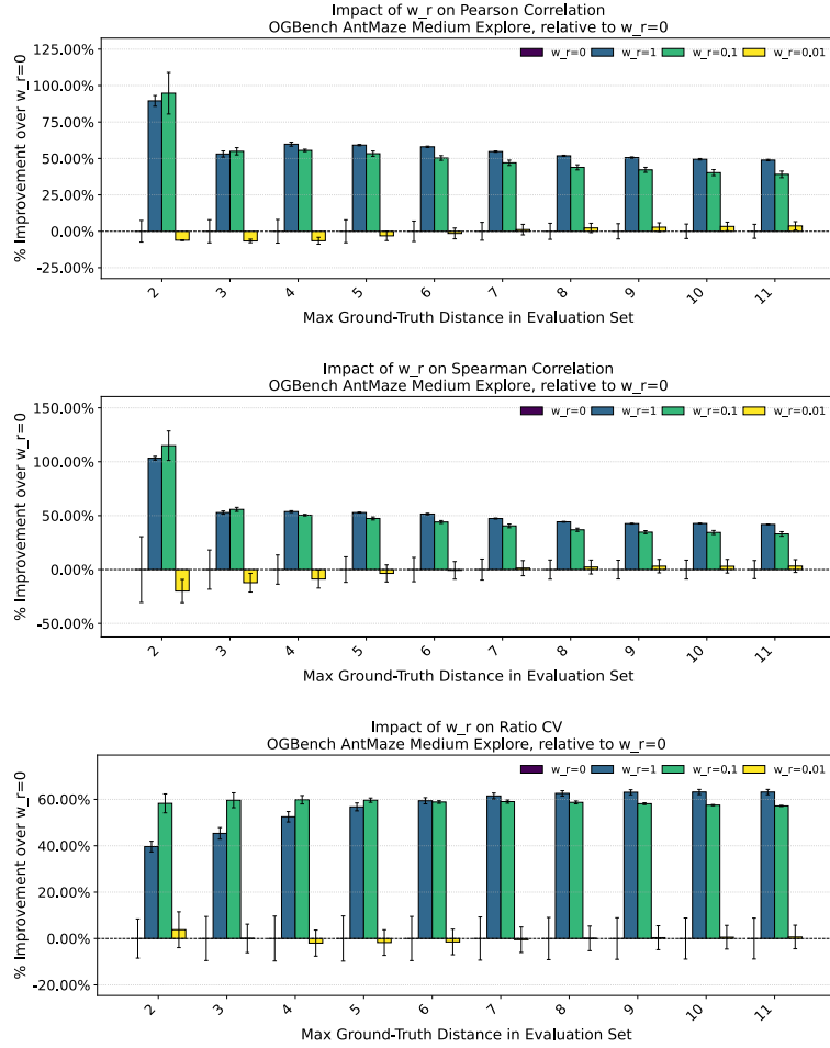
Figure 11. Impact of w_r on Pearson and Spearman correlation coefficients and coefficient of variation (CV) ratios on ogbench AntMaze Medium Explore
