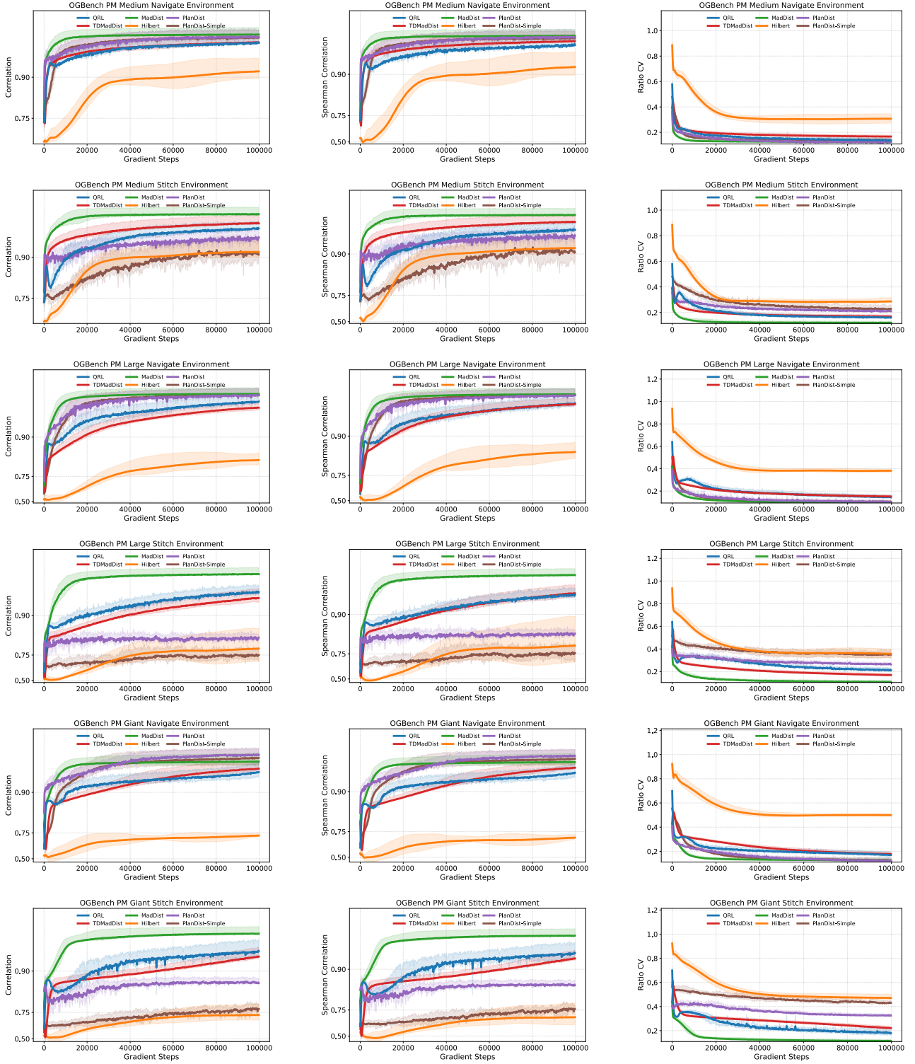
Figure 15. Pearson and Spearman correlation coefficients and coefficient of variation (CV) ratios across OGBench PointMaze test environments. Shaded regions show the range of values across five random seeds, with upper and lower boundaries representing maximum and minimum values.
