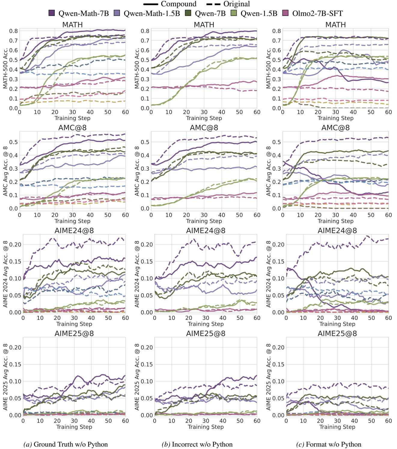
Figure 14. We present additional compound reward results on (1) smaller 1.5B Qwen models and (2) AMC and AIME benchmarks. See Section 5.3 for full details of the setup. Our compound rewards intersect (a) our original rewards with a (b) no Python reward that only rewards responses without Python code. Overall, our findings here are largely consistent with those from our main text. Note that AIME is a very small test set, so small differences in accuracy (less than \sim 2 percentage points) may not be meaningful.
