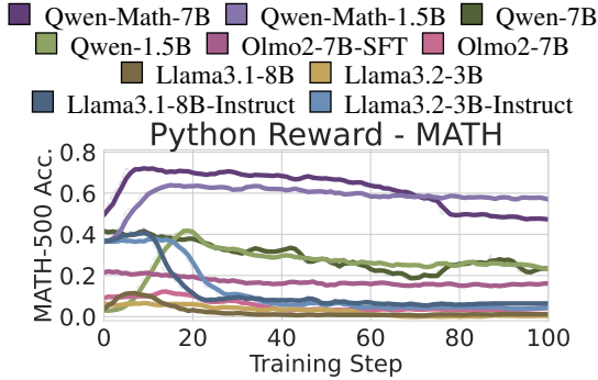
Figure 7. Performance when using our Python reward to explicitly encourage the model to perform code reasoning. This improves performance only in Qwen2.5-Math. Qwen2.5-Math-7B starts to generate > 99% code reasoning in 20 training steps.
