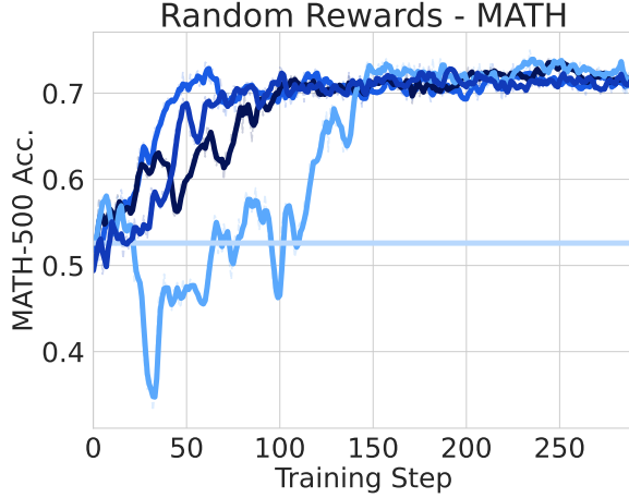
Figure 8. We train Qwen2.5-Math-7B using GRPO with random rewards of different probability \gamma \in \{0.7, 0.5, 0.3, 0.001, 0\} . We note that with the exception of \gamma = 0 , which leads the model to not perform any learning, all other probability configuration successfully leads the model to achieve a significant performance gain after some period of random walk. Furthermore, once in the high-accuracy regime, the training procedure maintain model’s performance.
