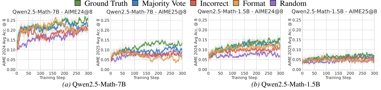
Figure 12. Qwen2.5-Math Model performance on AIME 2024 and AIME 2025.
