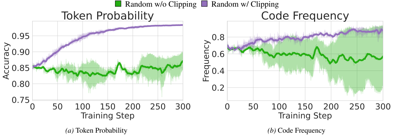
Figure 9. Token probability and code frequency of random rewards with (purple) and without (green) clipping on Qwen2.5-Math-7B.
