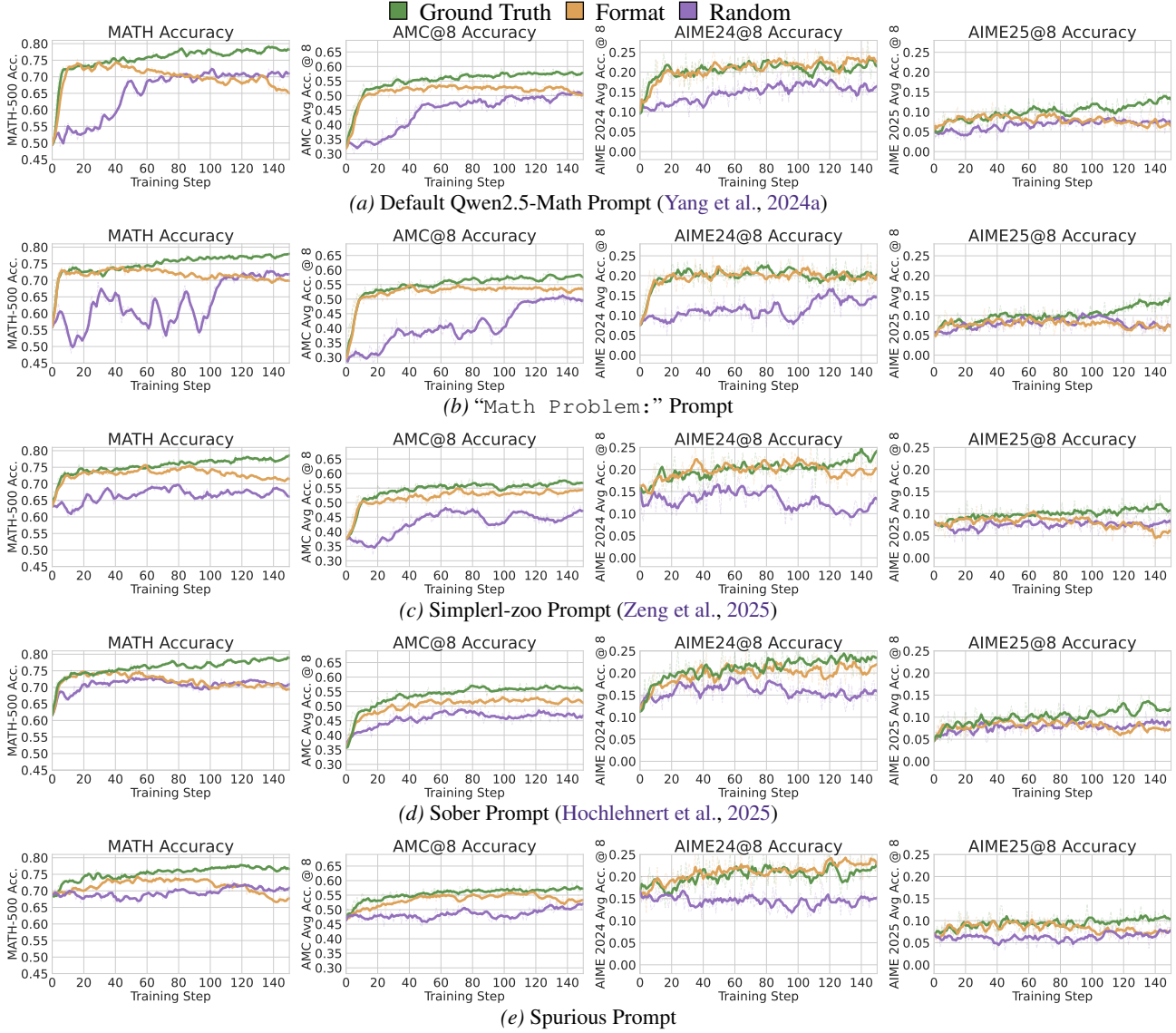
Figure 19. RLVR performance with different prompt templates on Qwen2.5-Math-7B. We show the choice of the prompt impacts both the before training performance and the RLVR training trajectories for Qwen2.5-Math-7B. We find the default prompt provided by Qwen2.5-Math (Yang et al., 2024a) results in lower initial performance; the other prompts offer higher initial performance, while Spurious Prompt offers the highest initial performance.
