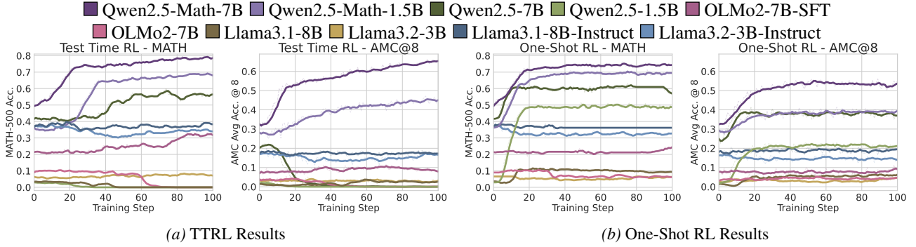
Figure 15. We evaluate two recent weak supervision RL methods—TTRL (Zuo et al., 2025) and One-Shot RL (Wang et al., 2025b)—on diverse base models. We find that the proposed training rewards can consistently work on Qwen models. Yet with few exceptions, those same proposed signals often yield no gains on other model families, mirroring the limited generalization observed when training with our own spurious rewards. See Appendix A.7 for setup details.
