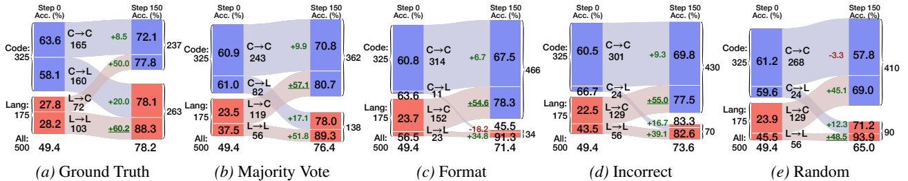
Figure 18. Reasoning strategy switching and fine-grained performance of Qwen2.5-Math-7B on the MATH-500 test set before and after RLVR with different training signals. Blue labels are the problem for which the model uses code reasoning, while red labels indicate reasoning traces using only natural language. Accuracy of each disjoint subset of problems before and after RLVR is shown in the shaded ends, and the size of each subset is shown in the lightly shaded region along with the change in accuracy. For all weak and spurious rewards, the model tends to use more code reasoning after RLVR. There is a small proportion of originally-code-reasoning problems being switched to language reasoning (Code→Lang); a majority of originally-language-reasoning problems convert to code reasoning (Lang→Code), on which we see the most significant performance increase after RLVR.
