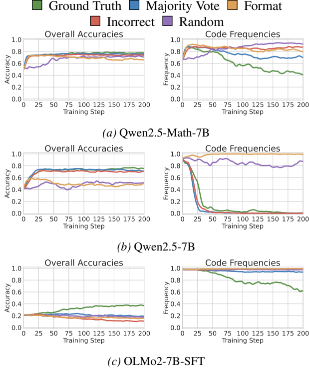
Figure 6. We track MATH-500 accuracy (left) and the proportion of answers containing Python code (right) for a Qwen2.5-Math-7B model trained with different reward signals. Under weak (format) or spurious (random, incorrect) rewards, both accuracy and code frequency increase. In contrast, training with ground-truth rewards improves accuracy while code frequency eventually declines, suggesting a different improvement mechanism.
