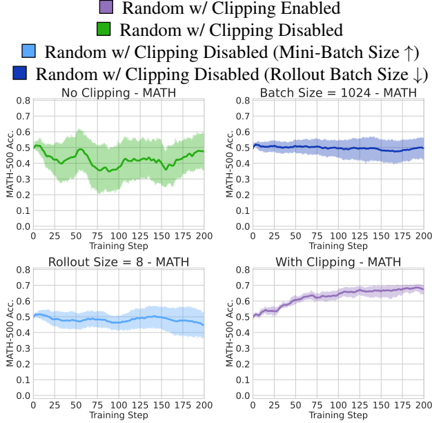
Figure 4. Average performance over multiple random seeds when ablating the clipping term in GRPO with random rewards for Qwen2.5-Math-7B. The first three panels correspond to no-clipping variants (see text), while the last panel enables clipping. Random rewards yield consistent improvements only when clipping is present.
