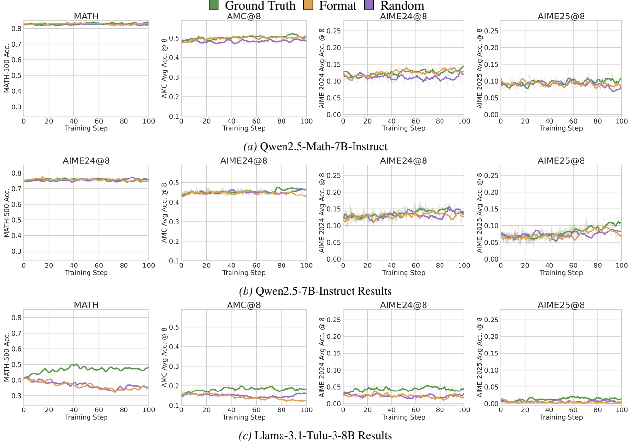
Figure 20. RLVR performance on models that have undergone RL training. We find that Qwen Instruct models show minimal improvement from our RLVR, while Llama-3.1-Tulu-3-8B exhibits similar patterns to OLMo models (Figure 3). There is a clear performance distinction when training with ground truth labels for Llama-3.1-Tulu-3-8B, but not for the Qwen Instruct models.
