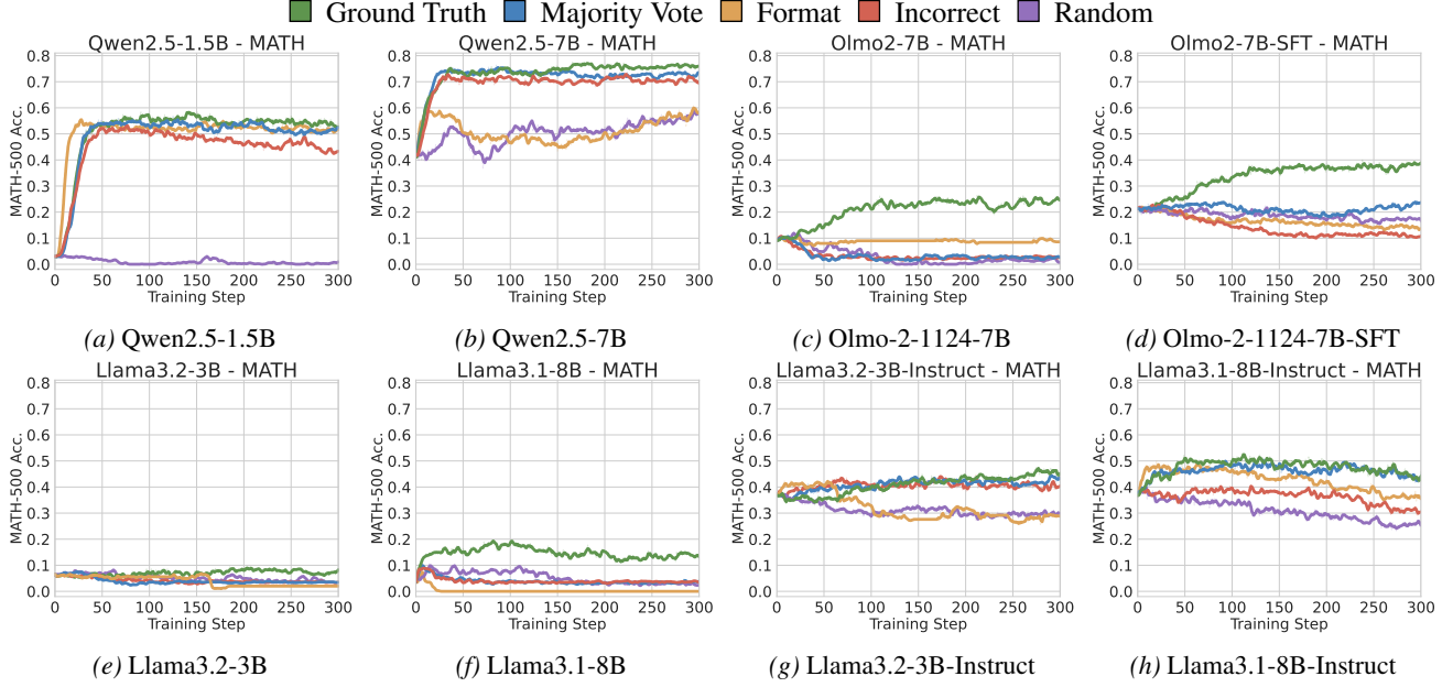
Figure 3. Varying rewards across additional model classes on MATH-500. Spurious rewards remain effective on general-purpose Qwen2.5 models but generally fail to yield any gains on other model families. The performance improvements on non-Qwen2.5 models are substantially smaller compared to those observed in the Qwen2.5 family. Similar trends are observed on AMC in Appendix C.
