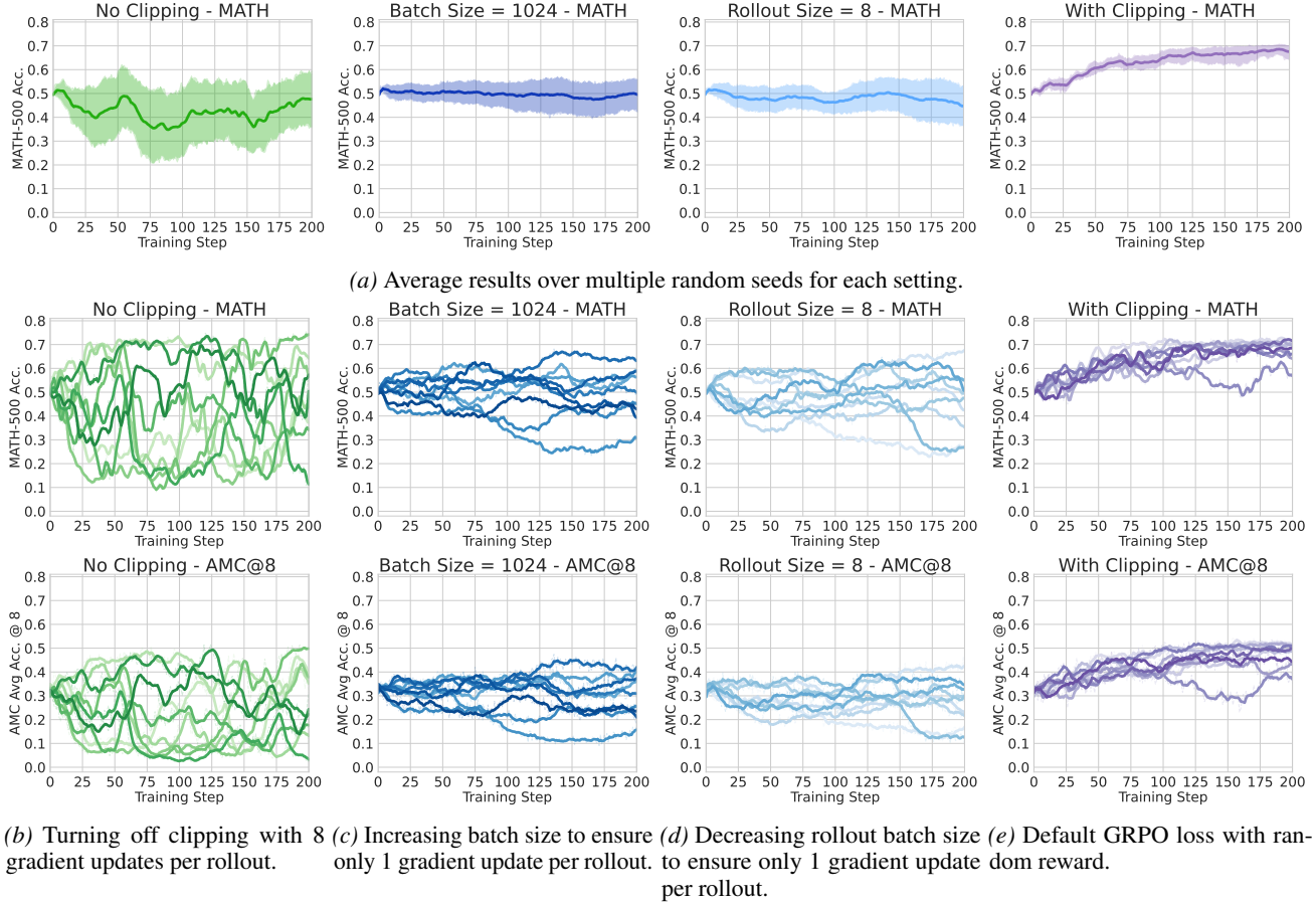
Figure 10. RLVR performance on random rewards with disabled clipping across multiple different seeds. Models without clipping show no meaningful performance improvement on average, while models with clipping demonstrate consistent performance gains using random rewards. Disabling clipping in implementation produces high variance in results, occasionally yielding high accuracy scores. Experiments with adjusted batch sizes exhibit greater stability but involve 8 times fewer gradient updates than the disabled clipping experiments.
