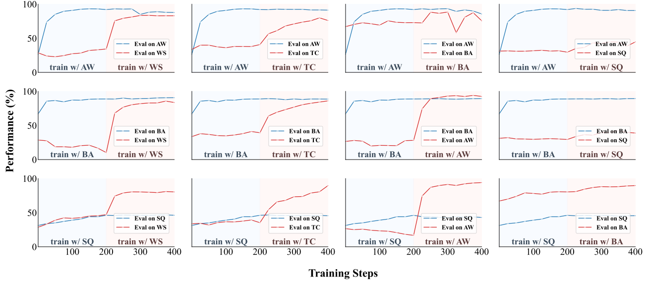
Figure 7. Training dynamics of forgetting and transfer in other sequential two-stage cross-environment training with Qwen2.5-7B-Instruct, where blue and red denote the upstream environment and the downstream environment, respectively.
