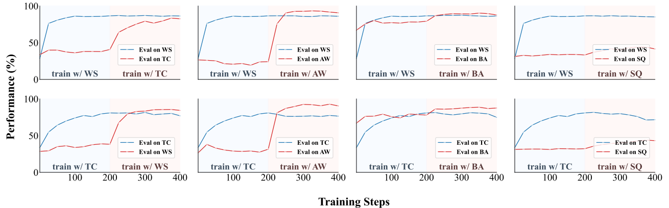
Figure 3. Training dynamics of forgetting and transfer in sequential two-stage cross-environment training with Qwen2.5-7B-Instruct, where blue and red denote the upstream environment and the downstream environment, respectively.
