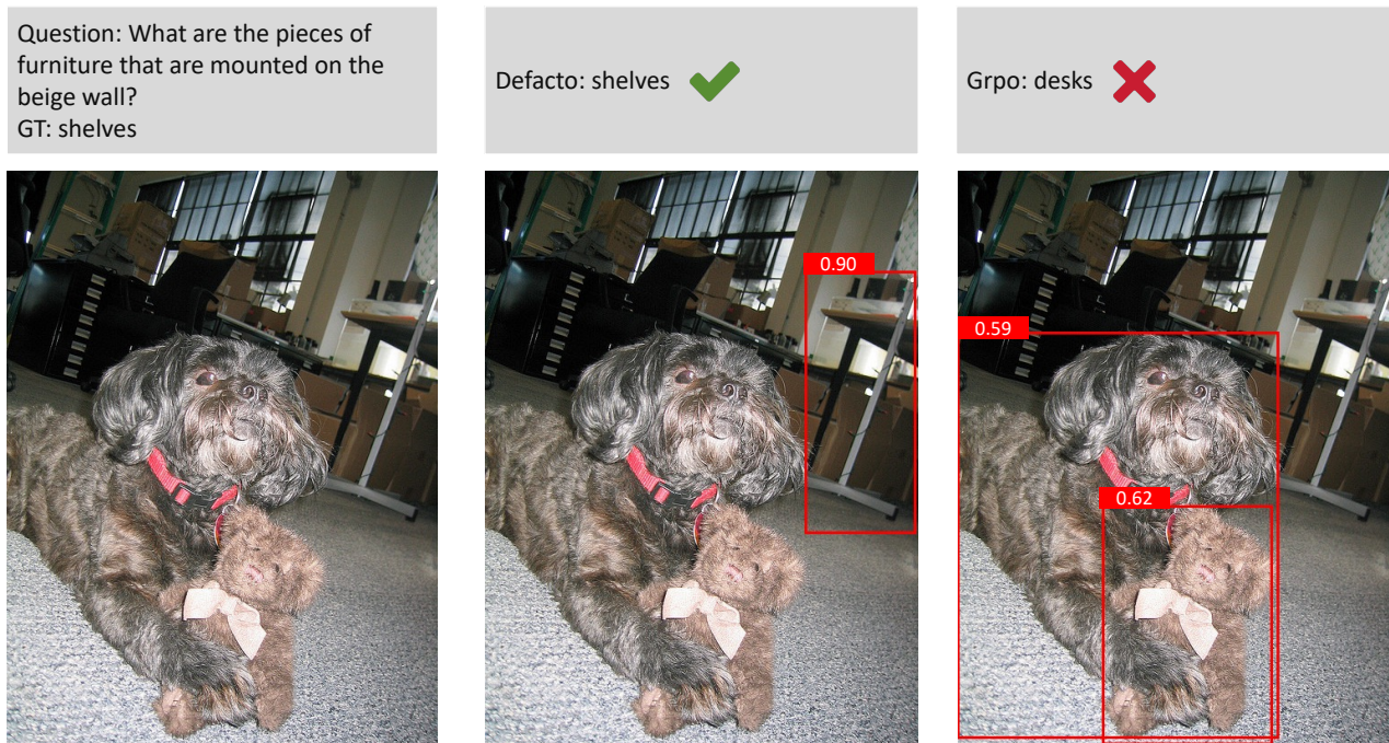
Figure 12. Visualization examples comparing DeFACTO and standard GRPO
