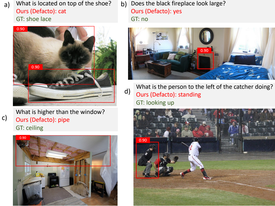
Figure 9. Four representative failure cases illustrating different types of semantic and perceptual ambiguities.
