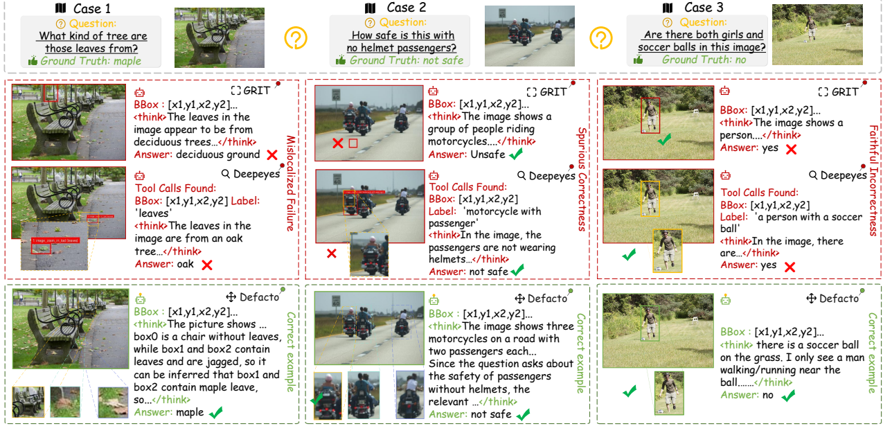
Figure 1. Qualitative examples of unfaithful reasoning in thinking-with-images. We categorize failures into three types: Mislocalized Failure (wrong evidence, wrong answer), Spurious Correctness (wrong evidence, correct answer), and Faithful Incorrectness (correct evidence, wrong answer). We compare two representative baselines (Deepeyes and GRIT) with our method on three cases.
