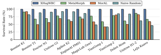
Figure 5. Zero-shot survival rate comparison across multiple baselines. All policies are trained under the same training protocol. Naive Random is trained on data generated by the naive morphological randomization method, whereas XHugWBC, MetaMorph, and MorAL are trained using randomization in Sec. 3.1.
