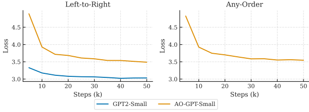
Figure 2. Validation loss curves during training comparing a standard AR GPT against an AO-GPT. Both models employ an identical decoder-only architecture, with AO-GPT demonstrating slower initial convergence.
