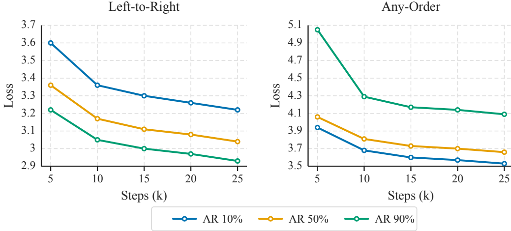
Figure 11. Ablation on left-to-right mixing ratio. We vary the fraction of left-to-right orders mixed into random-order training. Increasing the left-to-right ratio improves the left-to-right loss, but hurts the any-order loss, revealing a trade-off between left-to-right specialization and any-order modeling.
