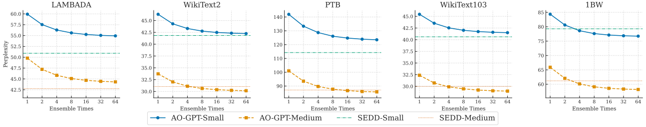
Figure 4. Zero-shot unconditional perplexity ( \downarrow ) for varying ensemble sizes. An ensemble size of 1 represents the baseline model without ensembling.
