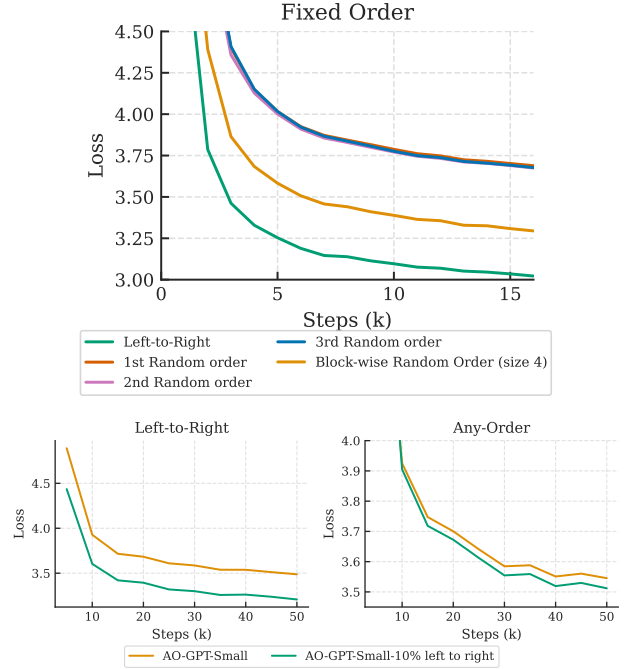
Figure 3. Top: Convergence speed with different fixed prediction orders: left-to-right, fixed random, and fixed block-wise random. Bottom: Impact of adding 10% left-to-right (L2R) data to AO-GPT training on its L2R and any-order loss. All losses reported in this figure are validation losses measured throughout training.
