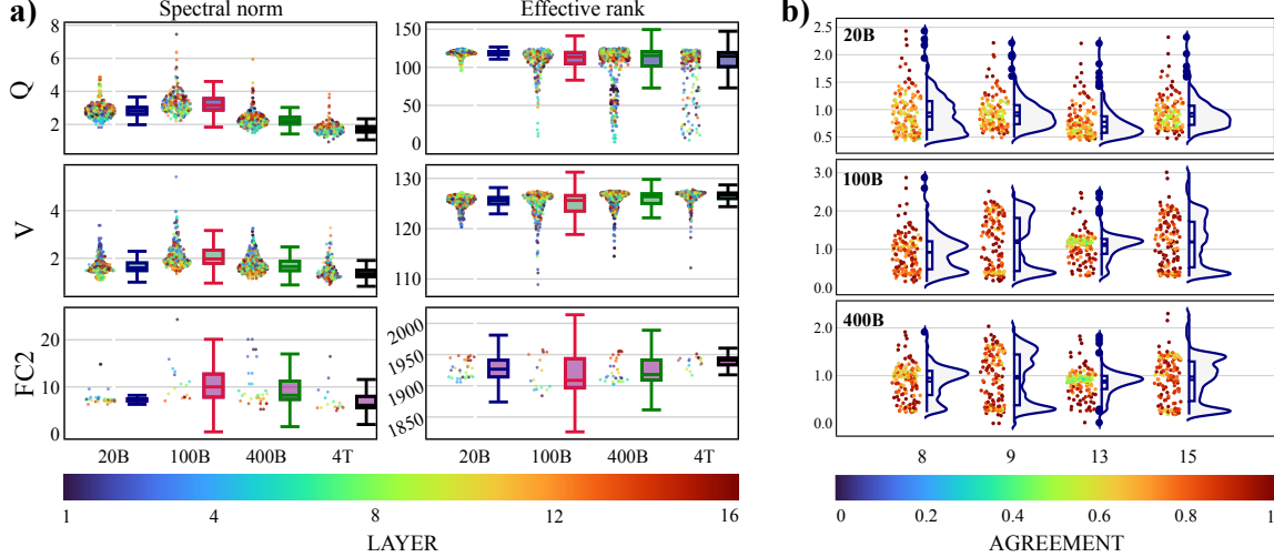
Figure 2. Spectral shape and metrics evolution during pre-train. a) Rows (top to bottom) correspond to W^Q , W^V , and W^{FC2} weight matrices, while columns (left to right) report the Spectral norm and the Effective rank. Each subplot overlays jittered per-matrix values with box plots summarizing the distributions for models pre-trained on 20B, 100B, 400B, and 4T tokens. Points denote individual matrices and are color-coded by the corresponding layer index. b) Singular value spectra for W^Q (layer 6, heads 8, 9, 13, 15) at 20B, 100B, and 400B tokens. Jitter points represent singular values and are colored by the left singular vector agreement between each pre-train checkpoint and the corresponding CPT endpoint on math domain. Note the increasingly complex spectral shape that poorly conforms to MP and PL models. Starting at 100B the singular vectors that change during the CPT stage are increasingly localized in narrow spectral bands.
