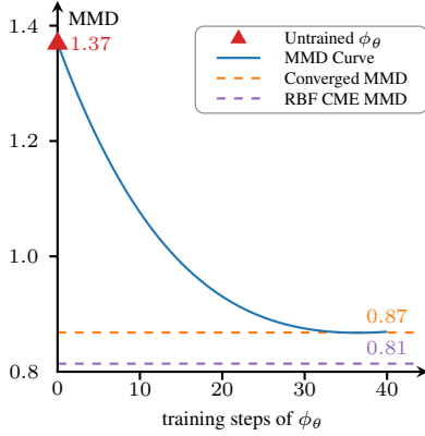
Figure 3. MMD from estimated to true CMEs over training steps of neural feature map \phi_\theta on a complex synthetic dataset.
