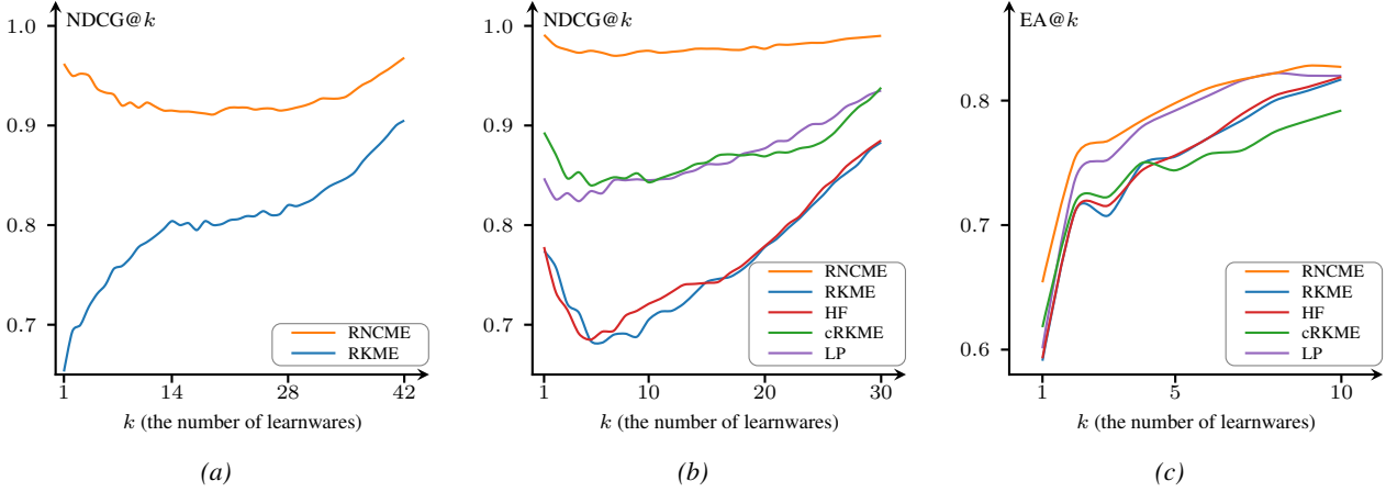
Figure 1. Experimental results on real-world regression and classification datasets: (a) NDCG@ k performance on California Housing Prices dataset across all k \leq n ; (b) NDCG@ k performance on NICO ++ dataset across all k \leq n ; (c) the average ensemble accuracy for top- k recommended learnwares on NICO ++ dataset across k \leq 10 .
