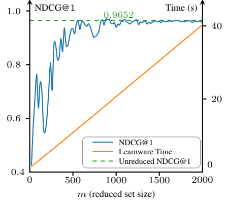
Figure 2. The time cost and recommendation performance (NDCG@1) of RNCME with varying reduced set size m on the California Housing Prices Dataset.
