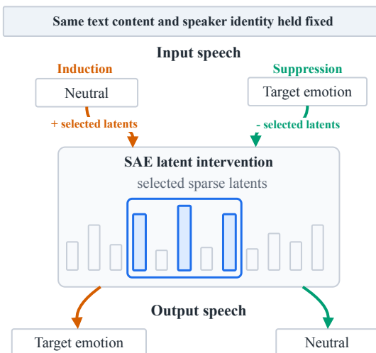
Figure 1. Conceptual overview of SAE-based bidirectional emotion control in the semantic backbone. Holding text content and speaker identity fixed, we intervene on selected SAE latent features. Increasing these features induces a target emotion from neutral speech, whereas decreasing them suppresses the target emotion toward neutral speech.
