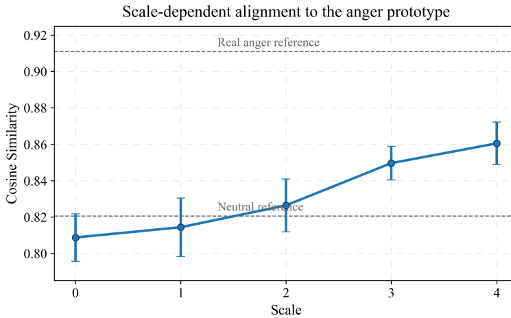
Figure 13. Emotion-prototype alignment under top-6 latent-feature steering in LLaSA. Cosine similarity is measured against the anger prototype; dashed lines denote neutral and real anger reference levels.
