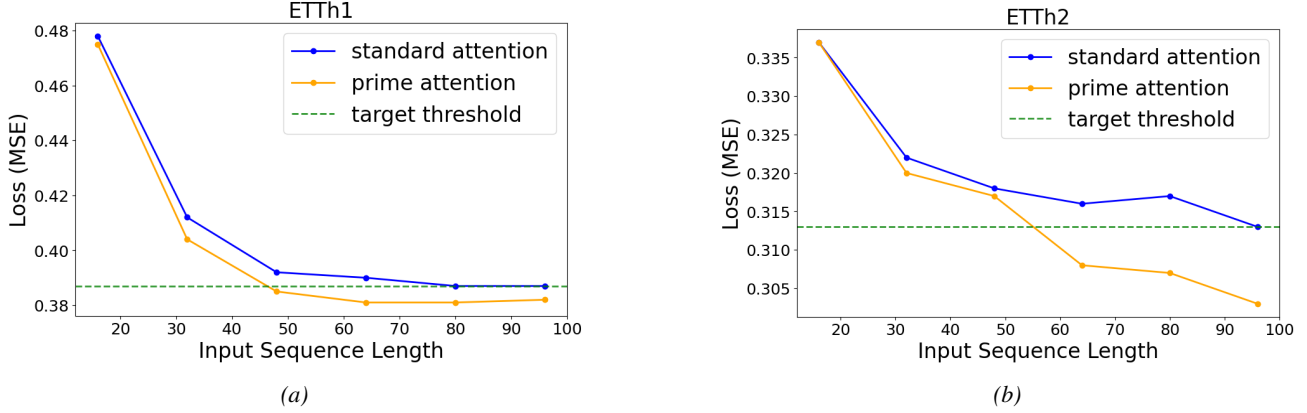
Figure 1. Comparing performance between standard (blue) and prime (yellow) attention at various input sequence length (or look-back window L ). The horizontal target threshold line (green, dotted) represents standard attention’s performance at L = 96 . Lower values indicate better performance.
