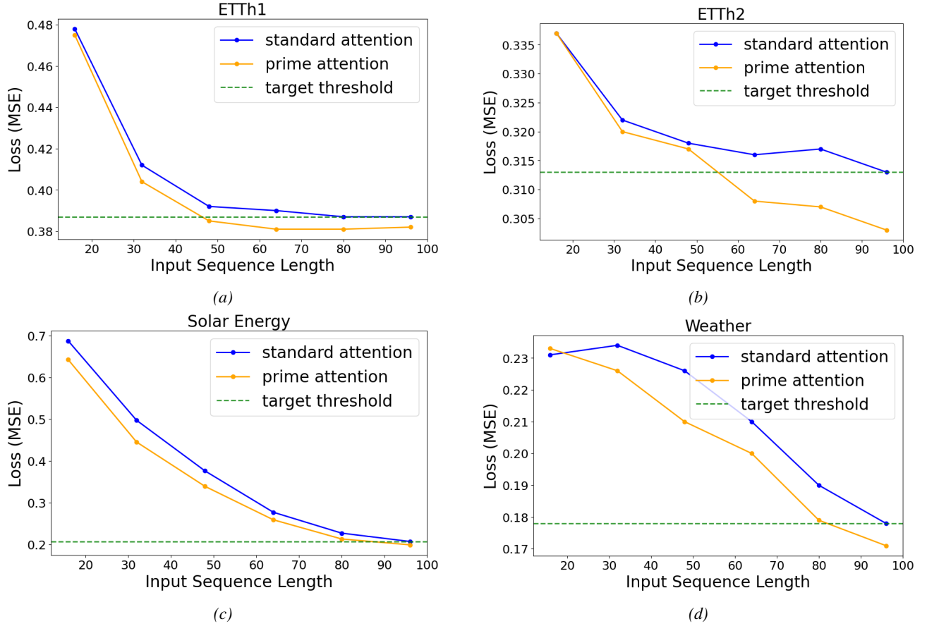
Figure 11. Comparing performance between standard (blue) and prime (yellow) attention at various input sequence length (or look-back window L ). The horizontal target threshold line (green, dotted) represents standard attention's performance at L = 96 .
