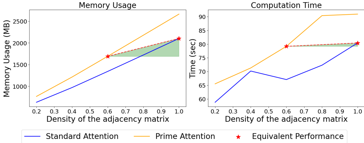
Figure 6. Analysis of memory (left) and computation time (right) for standard (blue) and prime (yellow) attention on the Weather dataset. The red star indicates observed equivalent performance (loss in MSE) between standard and prime attention.
