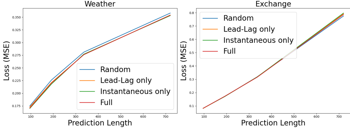
Figure 5. Effect that different initialization strategies for pair-wise modulation primer \mathcal{F} has on performance (y-axis, lower is better) across prediction lengths (x-axis).
