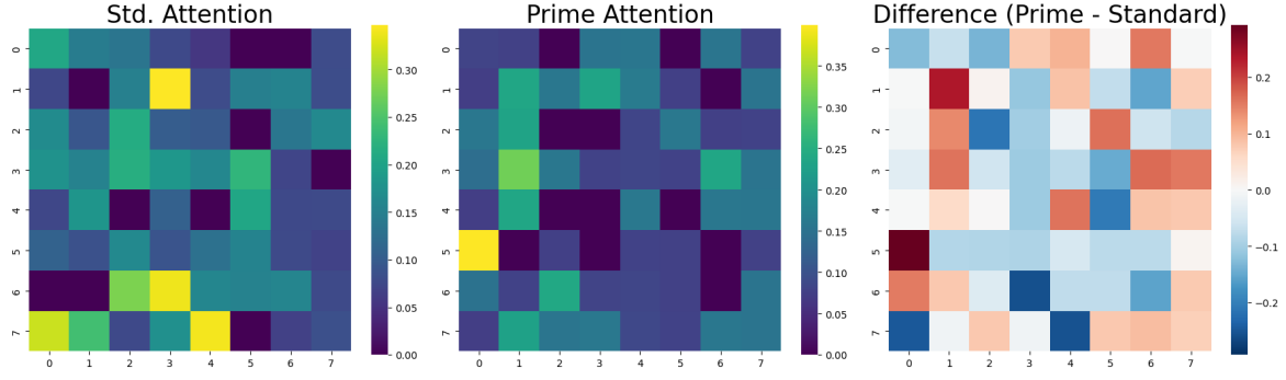
Figure 9. Attention maps of standard attention (left), prime attention (middle), and their difference (right) on the Exchange dataset. Warmer colors (yellow/green) reflect higher attention coefficient and colder colors (blue/purple) reflect lower attention coefficient.
