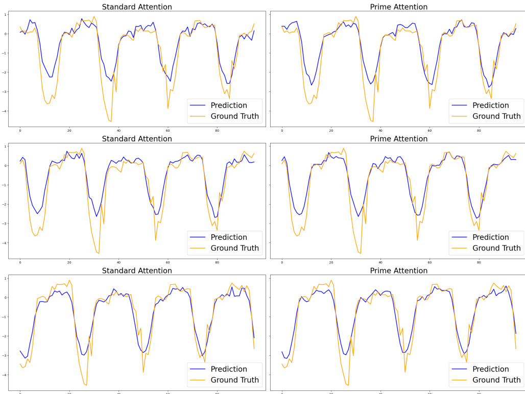
Figure 12. Forecasting visualization on ETTh1 dataset using predictions (in blue) made from standard attention (left) and prime attention (right) against ground-truth labels (in yellow). Each row represents a random batch.
