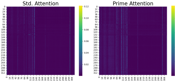
Figure 3. Attention map comparison between standard (left) and prime (right) attention on the ECL dataset. Despite being comparable in performance on this dataset, prime attention exhibits a more diverse attention pattern than standard attention, learning to focus on a larger number of channels compared to standard attention. This can be seen from the larger number of vertical lines present in prime attention’s attention map.
