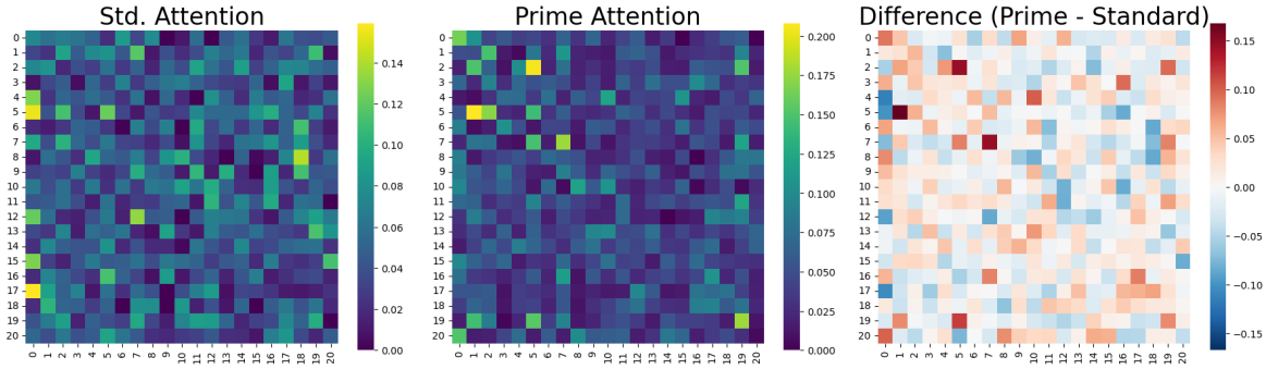
Figure 7. Attention maps of standard attention (left), prime attention (middle), and their difference (right) on the Weather dataset. Warmer colors (yellow/green) reflect higher attention coefficient and colder colors (blue/purple) reflect lower attention coefficient.
