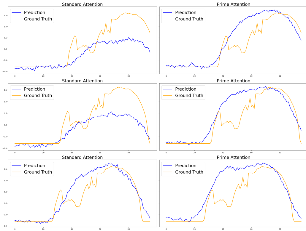
Figure 13. Forecasting visualization on Solar dataset using predictions (in blue) made from standard attention (left) and prime attention (right) against ground-truth labels (in yellow). Each row represents a random batch.
