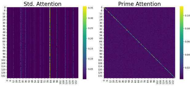
Figure 2. Attention map comparison between standard and prime attention on the Solar dataset. Standard attention (left) shows an over-reliance on a single channel (displayed as a yellow vertical line) which may indicate that the model is prematurely converging to an easy solution, unable to capture more diverse and complex patterns. Prime attention (right) on the other hand shows its ability to act as a soft CI model, learning to prioritize self-signals along the diagonal instead of developing an over-reliance on a single channel.
