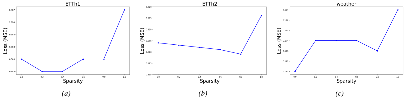
Figure 4. Ablation study on sparsity of pair-wise modulator \mathcal{F} . Sparsity refers to the amount (in percentage) of token pairs getting modulated (from left to right, 0% sparsity is full pair-wise modulation and 100% sparsity is equivalent to standard attention).
