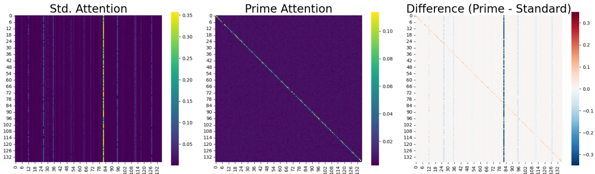
Figure 8. Attention maps of standard attention (left), prime attention (middle), and their difference (right) on the Solar dataset. Warmer colors (yellow/green) reflect higher attention coefficient and colder colors (blue/purple) reflect lower attention coefficient.
