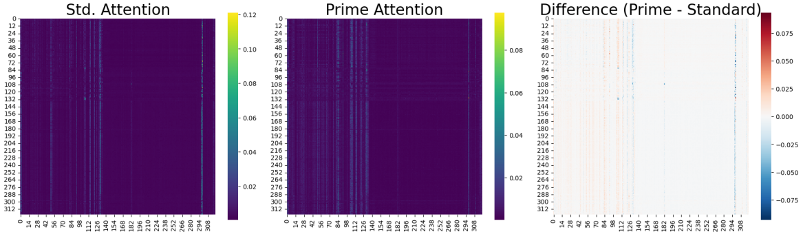
Figure 10. Attention maps of standard attention (left), prime attention (middle), and their difference (right) on the ECL dataset. Warmer colors (yellow/green) reflect higher attention coefficient and colder colors (blue/purple) reflect lower attention coefficient.
