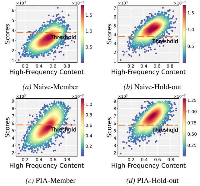
Figure 1. Statistical plots of membership scores versus high-frequency content for the MS-COCO dataset. Horizontal coordinates indicate high-frequency content, and vertical coordinates indicate membership scores. We used red to indicate areas with the highest data density.
