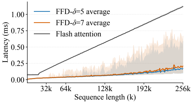
Figure 3. Kernel Latency vs. Sequence Length (RTX 4090). Layer-averaged execution time for FlashAttention-2 and FFD variants (batch=1). FFD- \delta = 5 and \delta = 7 achieve average speedups of 7.33\times and 6.18\times respectively, with a peak reduction of 11.63\times . Error bands denote the min-max range across layers.
