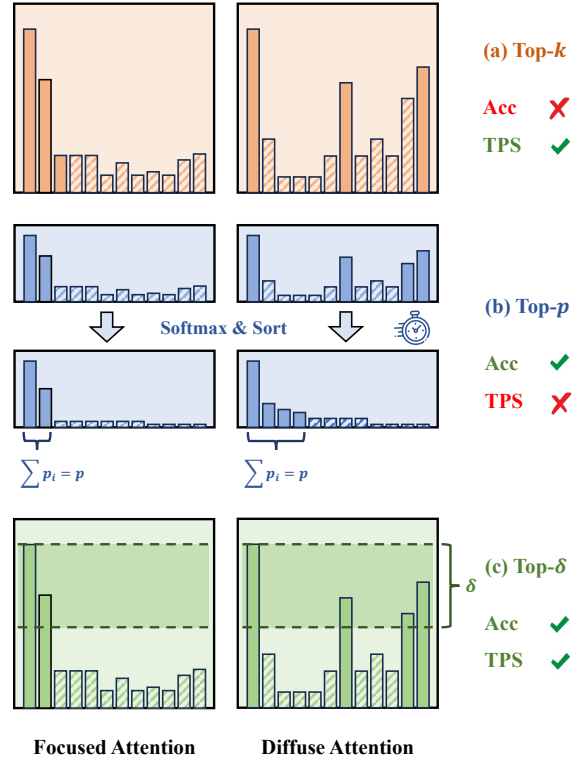
Figure 1. Comparison of selection strategies. (a) Top- k (fixed budget) is fast but fails to adapt to distribution shape. (b) Top- p offers dynamic cardinality but introduces non-trivial overhead due to global synchronization and sorting, which breaks the streaming pipeline. (c) Top- \delta (ours) uses a relative threshold \delta from the local max, achieving the adaptivity of top- p with the hardware efficiency of top- k .
