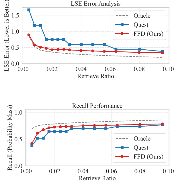
Figure 6. Quality vs. IO Budget on Llama. FFD maintains lower LSE error while achieving higher recall than Quest under the same retrieval budget, showing that high-fidelity scanning preserves distributional accuracy and hit rate.
