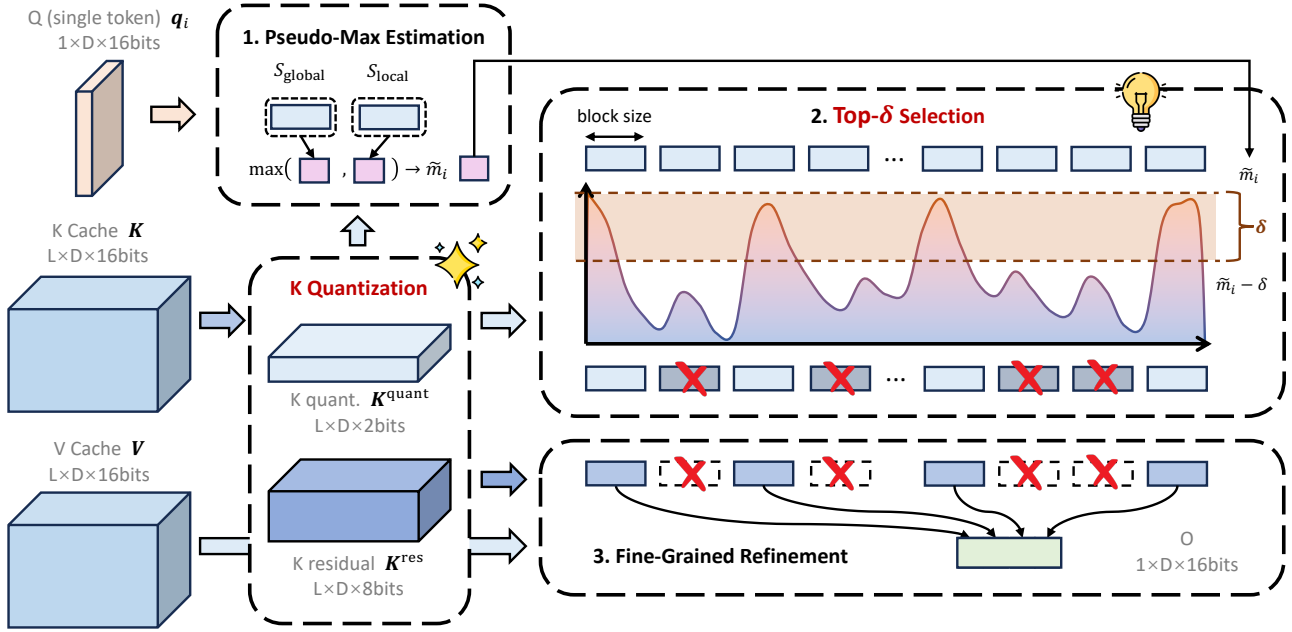
Figure 2. Overview of our FFD implementation. Inputs include the 16-bit query as well as the value cache and the key cache split into a 2-bit quantized thumbnail and an 8-bit residual. The attention output is acquired after K quantization, pseudo-max estimation, top- \delta selection, as well as filtering based on the top- \delta strategy, and fine-grained refinement.
