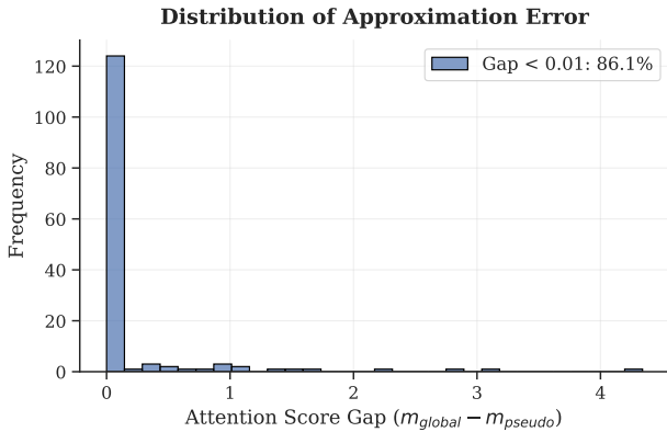
Figure 5. Distribution of the approximation error ( m_i - \tilde{m}_i ) by layer. The gap is effectively zero for most of conditions, confirming that the maximum attention score is dominated by sinks and local tokens. This verifies that our Pseudo-Max approximation serves as a robust safe relaxation.
