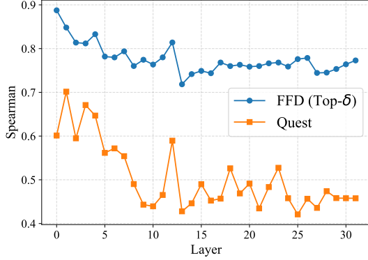
Figure 7. Layer-wise Correlation Trends. FFD achieves consistently higher Spearman correlations across all layers compared to Quest, indicating better preservation of the attention distribution’s structural properties.
